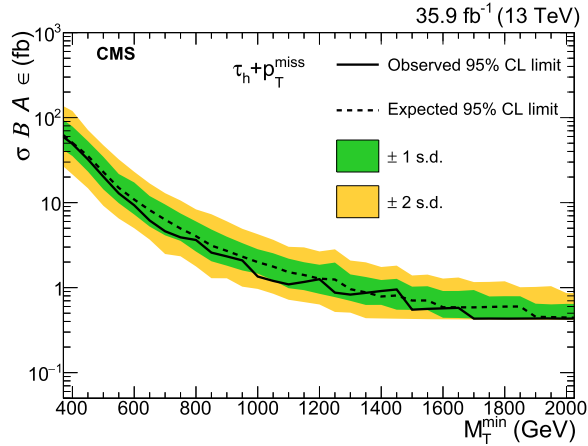
Fig. 8. Expected (black dashed line) and observed (black solid line) 95% CL model-independent upper limits on the product of cross section, branching fraction, and acceptance for a resonance decaying into the \tau\nu channel. The shaded bands represent the one and two standard deviation (s.d.) uncertainty bands.
