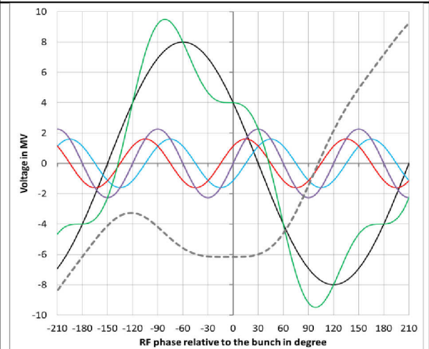
Fig. 9.6: Brightness mode bunch pattern with 80x20 bunches I_B = 200 \text{ mA} , P_{HHG} = 134 \text{ kW} , \phi_{HHG} = 0^\circ , \beta = 5.3 , \varphi_{HHC} = 45.3^\circ
