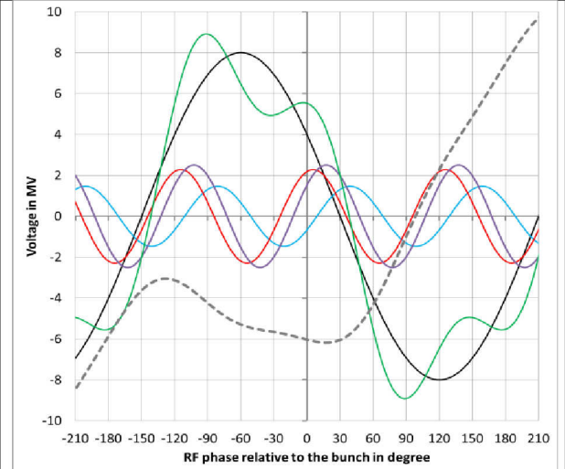
Fig. 9.4: Uneven bunch pattern. Half ring filled with 40x20 bunches I_B = 100 \text{ mA} , P_{HHG} = 71 \text{ kW} , \phi_{HHG} = 0^\circ , \beta = 5.3 , \varphi_{HHC} = 26.8^\circ
