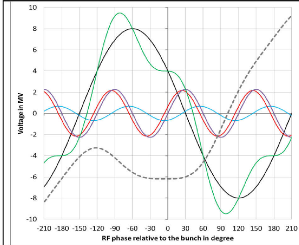
Fig. 9.1: Brightness mode bunch pattern with 80x20 bunches I_B = 200 \text{ mA} , P_{HHG} = 71 \text{ kW} , \phi_{HHG} = 0^\circ , \beta = 1 , \varphi_{HHC} = 72.5^\circ
