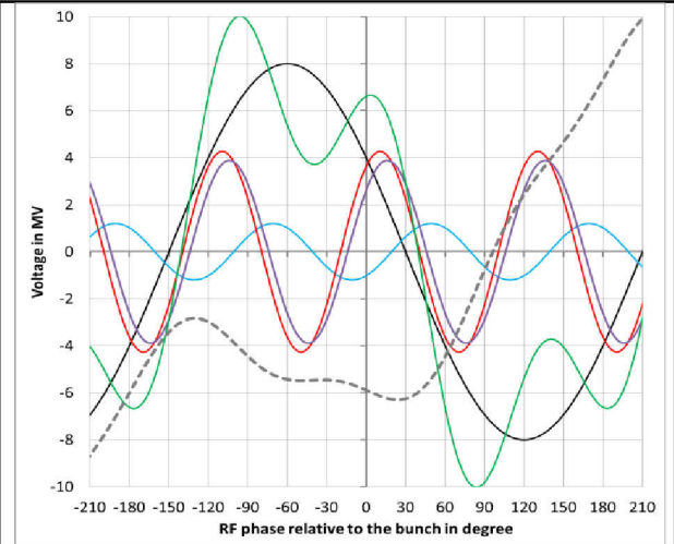
Fig. 9.2: Uneven bunch pattern. Half ring filled with 40x20 bunches I_B = 100 \text{ mA} , P_{HHG} = 71 \text{ kW} , \phi_{HHG} = 0^\circ , \beta = 1 , \varphi_{HHC} = 57.8^\circ
