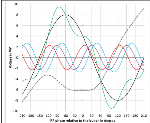
Fig. 9.5: Uneven bunch pattern. Half ring filled with 40x20 bunches I_B = 100 \text{ mA} , P_{HHG} = 240 \text{ kW} , \phi_{HHG} = -27^\circ , \beta = 5.3 , \varphi_{HHC} = 26.8^\circ
