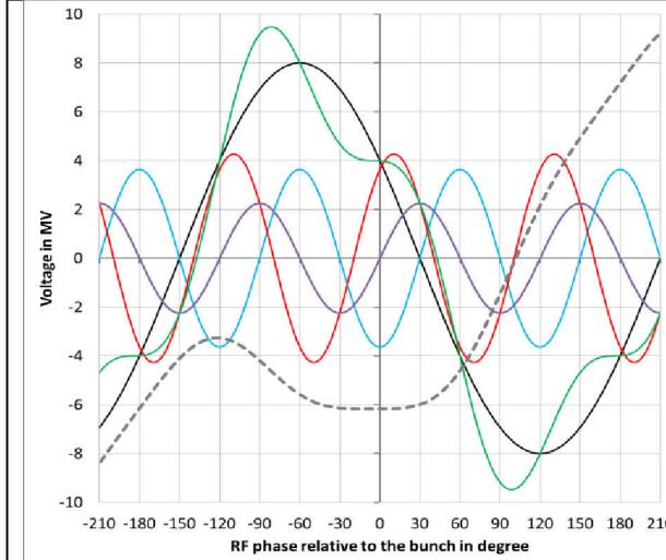
Fig. 9.3: Uneven bunch pattern. Half ring filled with 40x20 bunches I_B = 100 \text{ mA} , P_{HHG} = 650 \text{ kW} , \phi_{HHG} = -32^\circ , \beta = 1 , \varphi_{HHC} = 57.8^\circ
