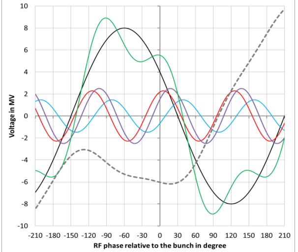
Fig. 9.4: Uneven bunch pattern. Half ring filled with 40x20 bunches I_B = 100 \text{ mA} , P_{HHG} = 71 \text{ kW} , \phi_{HHG} = 0^\circ , \beta = 5.3 , \varphi_{HHC} = 26.8^\circ
