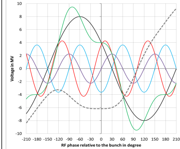
Fig. 9.3: Uneven bunch pattern. Half ring filled with 40x20 bunches I_B = 100 \text{ mA} , P_{HHG} = 650 \text{ kW} , \phi_{HHG} = -32^\circ , \beta = 1 , \varphi_{HHC} = 57.8^\circ
