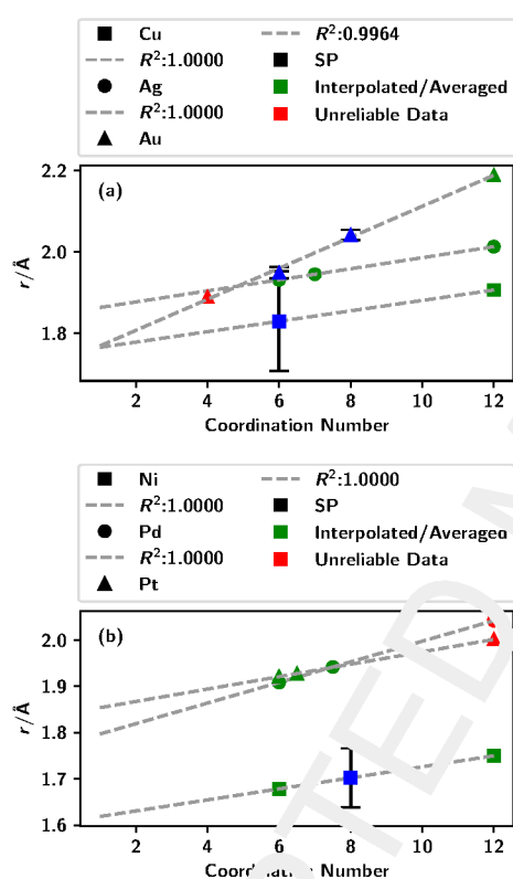
Figure 3: Influence of Coordination Number on r_{\text{ionic}} for group XI - (a) and X^{2-} (b) anions. While the available reference compounds allow for an evaluation of Au - with good accuracy, the evaluation of other elements is limited by the small sample size of appropriate binary compounds.
