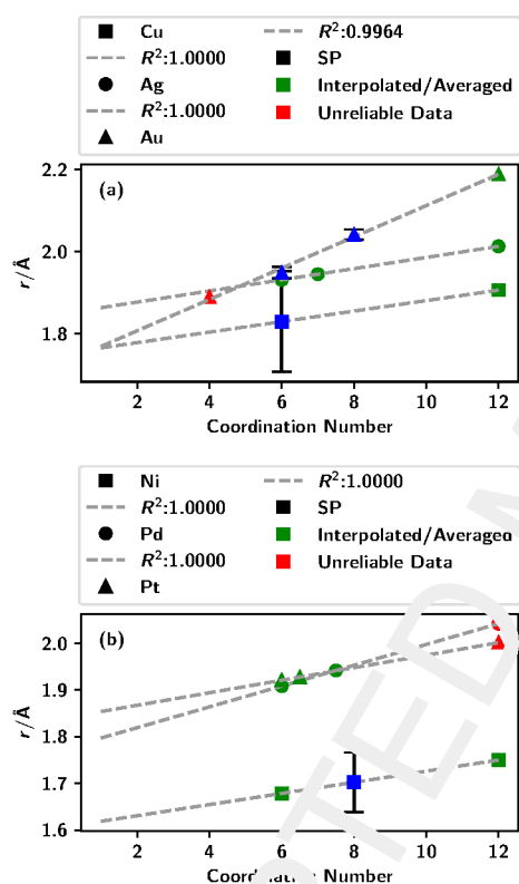
Figure 3: Influence of Coordination Number on r_{\text{ionic}} for group XI - (a) and X 2- (b) anions. While the available reference compounds allow for an evaluation of Au - with good accuracy, the evaluation of other elements is limited by the small sample size of appropriate binary compounds.
