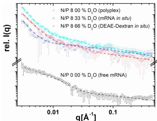
Fig. 6. SANS data of DEAE-Dextran-mRNA polyplexes (1.6 mg/ml) in HBGx1 buffer (pH 7.2). Plot shows measured scattering curves of particles at an N/P ratio of 8 at different H_2O/D_2O mixing ratios, as well as pure mRNA at 0% D_2O concentration (black curve). Dashed curves are fit models of the respective scattering curves obtained with SASfit using the unified exponential power law from Beaucage . Data are shifted vertically for clarity.
