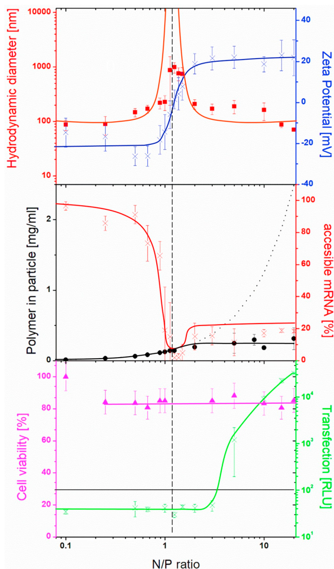
Fig. 2. Characterization of DEAE-Dextran/mRNA polyplexes. Top: hydrodynamic diameter (red line) and zeta potential (blue line) changes with respect to N/P ratio of DEAE-Dextran/mRNA polyplexes. Particle aggregation is observable at the inflection point of the sigmoidal zeta potential behavior (vertical black dashed line). Middle: Concentration of DEAE-Dextran in the particle (black dots). The free DEAE-Dextran was measured and subtracted from the total amount of DEAE-Dextran (black dots). In red: free accessible mRNA as measured from the Quant-it Ribogreen assay according to N/P ratio. Bottom: Cell viability (pink) and transfection (green) of DEAE-Dextran/mRNA polyplexes with respect to N/P ratio. All lines are drawn to guide the eye and do not represent any type of model fit. (For interpretation of the references to colour in this figure legend, the reader is referred to the Web version of this article.)
