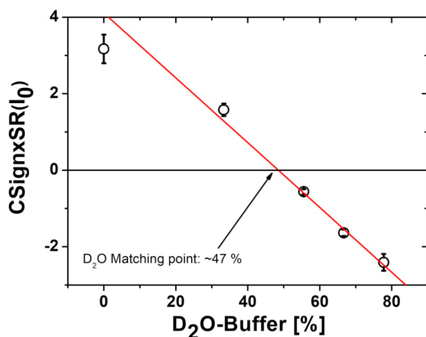
Fig. 7. Contrast matching point analysis. I_0 was obtained by extrapolating the scattering curve at low q values. The square root of I_0 plotted against the D_2O concentration in buffer yield the D_2O matching point and scattering length densities of DEAE-Dextran/mRNA polyplexes. The D_2O matching point is 47 \pm 3\% .
