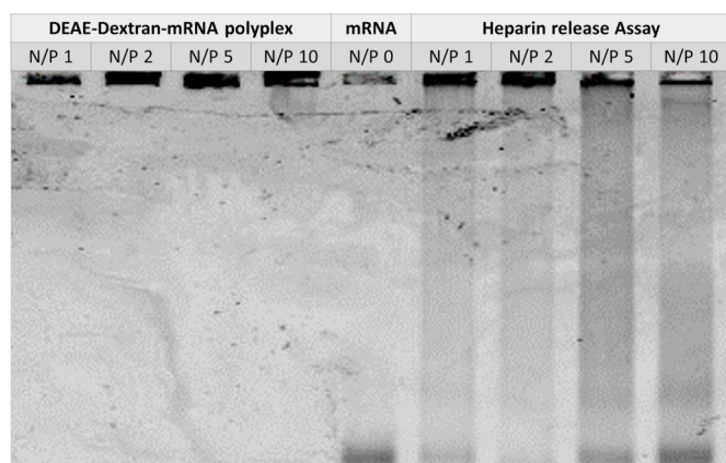
Fig. 3. Gel electrophoresis of DEAE-Dextran/mRNA polyplexes before (left) and after (right) Heparin release assay. mRNA bands are visible in different intensities after release. Positive control (mRNA) is the same mRNA in the same concentration as in the particles.
