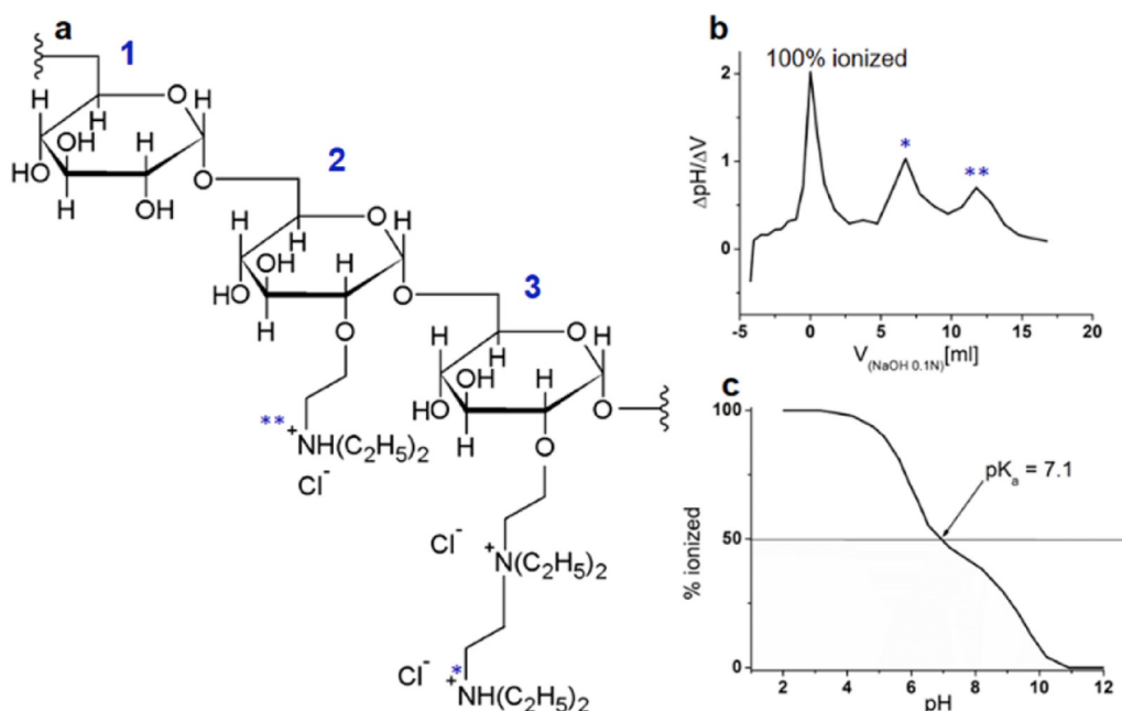
Fig. 1. a) Chemical Structure of DEAE-Dextran. Three different monomers are observable (1, 2, 3). The potentiometric titration reveals a proportion between the monomers of 6:1:1. Molecular weight is approx. 40 kDa. A total of 200 monomers is estimated. b) \Delta\text{pH}/\Delta V of 1.0 g DEAE-Dextran. * shows the peak position of the weaker tertiary amine, ** of the stronger tertiary amine. c) Ionization of the tertiary amines of DEAE-Dextran. The pKa of the two tertiary amines is 7.1. The amount of nitrogen is 2.72% in dry mass.
