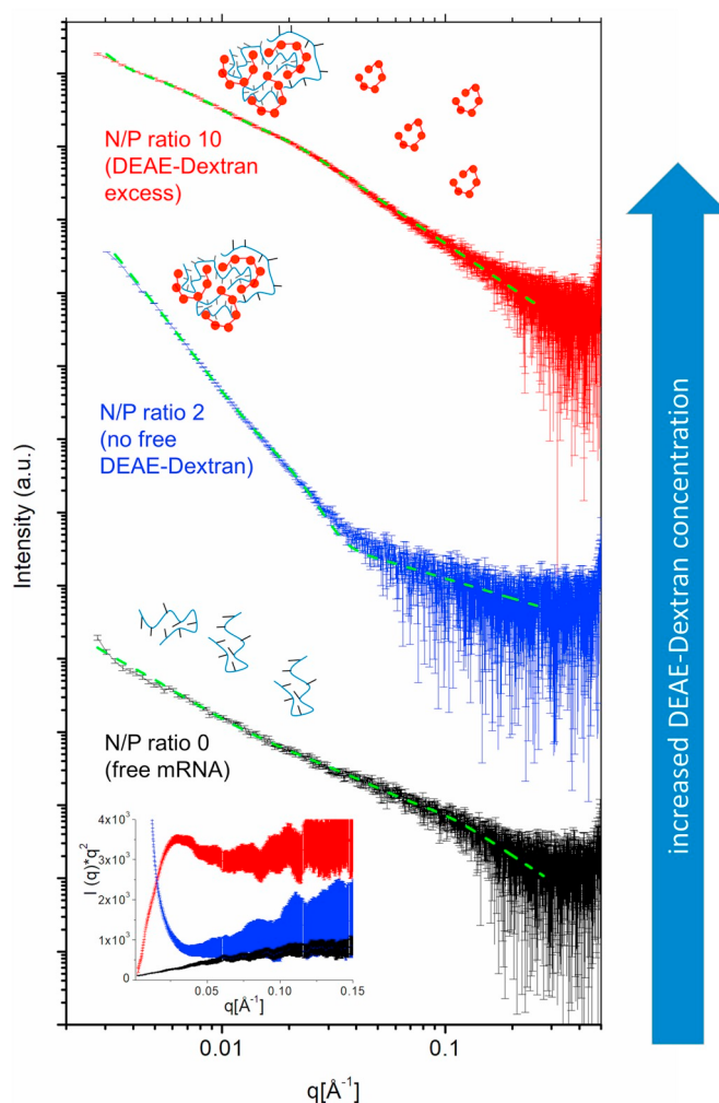
Fig. 4. SAXS data of DEAE-Dextran/mRNA polyplexes with an N/P ratio of 0 (black), 2 (blue) and 10 (red) in HBGx1 buffer (pH 7.2). Green dashed curves are fit models of the respective scattering curves obtained with SASfit using the unified exponential power law from Beaucage [38,39]. Data are shifted vertically for clarity. Kratky plot (bottom left inset plot) was obtained by plotting I(q) \cdot q^2 against q . (For interpretation of the references to colour in this figure legend, the reader is referred to the Web version of this article.)
