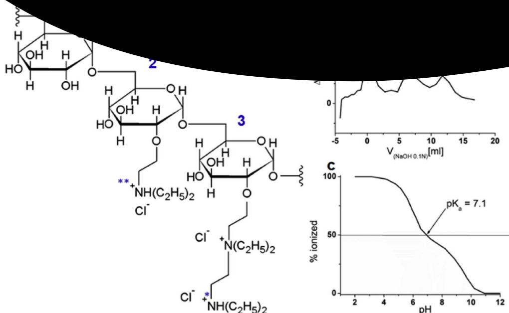
Fig. 1. a) Chemical structure of DEAE-Dextran. The molecular weight is approx. 40 kDa. A total of 200 monomers is estimated. b) \Delta pH/\Delta V of 1.0 g DEAE-Dextran. * shows the peak position of the weaker tertiary amine, ** of the stronger tertiary amine. c) Ionization of the tertiary amines of DEAE-Dextran. The pK a of the two tertiary amines is 7.1. The amount of nitrogen is 2.72% in dry mass.
