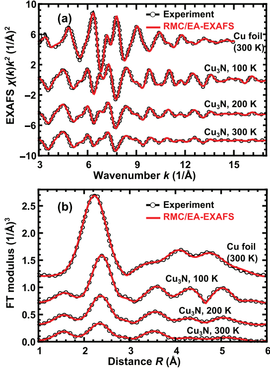
Figure 3: (Color online) Comparison between the experimental (open circles) and calculated (solid lines) Cu K-edge EXAFS spectra (a) and their Fourier transforms (b) for metallic copper at 300 K and for \text{Cu}_3\text{N} at 100, 200 and 300 K. Calculated configuration-averaged Cu K-edge EXAFS spectra correspond to the final RMC/EA configuration. Plots are shifted vertically for clarity.
