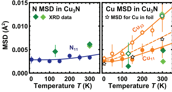
Figure 7: (Color online) Temperature dependencies of anisotropic MSD factors for N and Cu atoms in \text{Cu}_3\text{N} . \text{Cu}_{11} correspond to \langle u_{11}^2 \rangle MSD factor of copper, \text{Cu}_{33} correspond to \langle u_{22}^2 \rangle = \langle u_{33}^2 \rangle MSD factors of copper, \text{N}_{11} correspond to \langle u_{11}^2 \rangle = \langle u_{22}^2 \rangle = \langle u_{33}^2 \rangle MSD factors of nitrogen. Solid lines show the fits by the Einstein model. Dashed line shows the calculated 2(1/\langle u_{11}^2 \rangle + 1/\langle u_{33}^2 \rangle)^{-1} value, which corresponds to the MSD factor in the direction of the bond between two nearest Cu atoms. Diamonds show results from diffraction experiments [21] (light solid and open diamonds) and [20] (dark solid and open diamonds). The MSD values for Cu atoms in metallic copper are shown by open asterisks for comparison.
