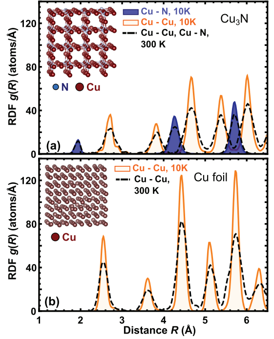
Figure 4: (Color online) Results of RMC/EA simulations for \text{Cu}_3\text{N} (a) and for metallic copper (b) at 10 K: the final structure models and partial Cu-Cu and Cu-N radial distribution functions (RDFs). The partial Cu-Cu and Cu-N RDFs at 300 K are also shown for comparison by dashed lines.
