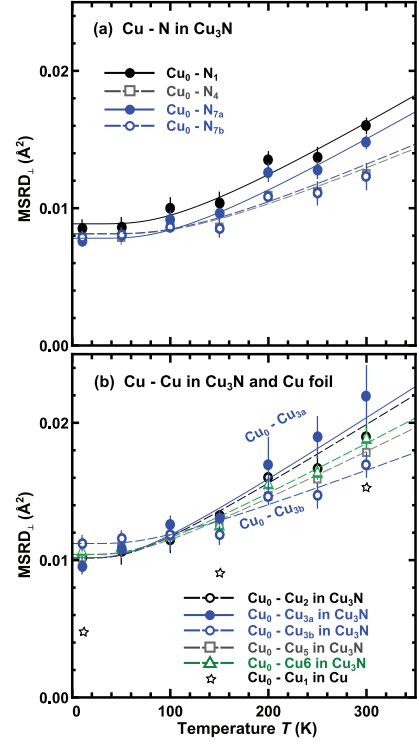
Figure 6: (Color online) Temperature dependencies of the perpendicular MSD factors for Cu-N (a) and Cu-Cu (b) atom pairs in the first seven coordination shells in Cu 3 N. Solid symbols refer to the atom pairs within single -N-Cu-N- chain, while open symbols – to the atoms in the off-chain positions. The data for the nearest neighbours in metallic copper are shown for comparison by open asterisks. Solid and dashed lines are the fits by the correlated Einstein model for atom pairs within single -N-Cu-N- chain and in the off-chain positions, respectively.
