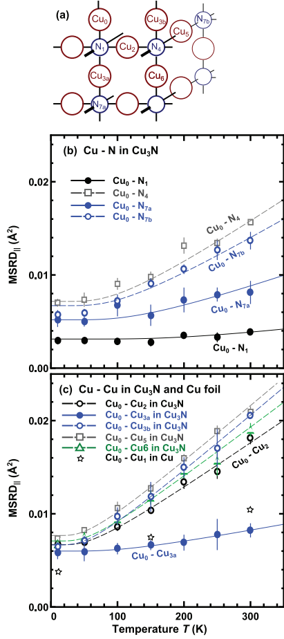
Figure 5: (Color online) (a) A fragment of the Cu 3 N structure. Atoms of the nearest seven coordination shells around the absorbing copper Cu 0 are indicated. Temperature dependencies of the parallel MSD factors for Cu-N (b) and Cu-Cu (c) atom pairs in the first seven coordination shells in Cu 3 N. Solid symbols refer to the atom pairs within single -N-Cu-N- chain, while open symbols – to the atoms in the off-chain positions. The data for the nearest neighbours in metallic copper are shown for comparison by open asterisks. Solid and dashed lines are the fits by the correlated Einstein model for atom pairs within single -N-Cu-N- chain and in the off-chain positions, respectively.
