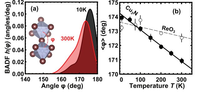
Figure 9: (Color online) Temperature dependencies of (a) the N-Cu-N angle distribution and (b) the average N-Cu-N angle value (solid circles) in \text{Cu}_3\text{N} . The values of the Re-O-Re angle in perovskite-type \text{ReO}_3 (from [52]) are shown for comparison in (b). Solid and dashed lines – guides for the eye.
