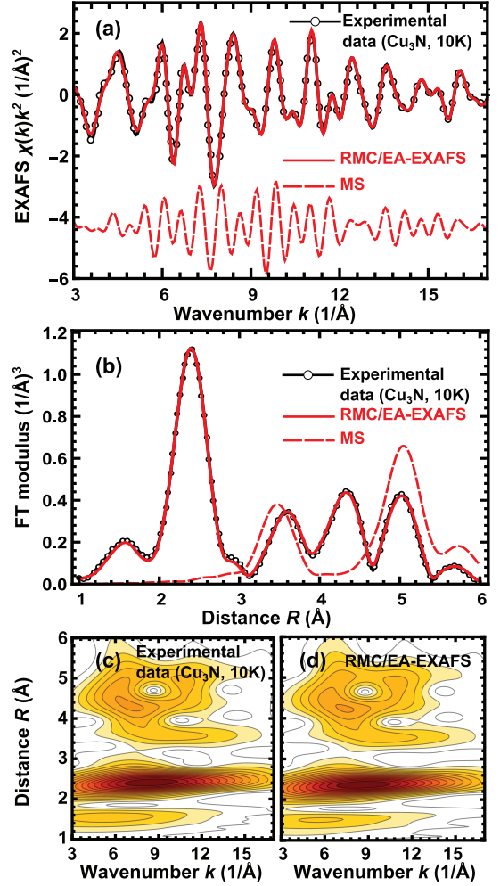
Figure 2: (Color online) Comparison of the experimental ( T = 10 K) and calculated configuration-averaged Cu K-edge EXAFS spectra of \text{Cu}_3\text{N} (a) and their Fourier (b) and Morlet wavelet (c, d) transforms. Dashed lines in panel (a) and (b) show the multiple-scattering contribution to the total calculated EXAFS spectrum and its FT. Spectra in panel (a) are shifted vertically for clarity.
