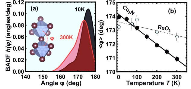
Figure 9: (Color online) (Color online) Temperature dependencies of (a) the N-Cu-N angle distribution and (b) the average N-Cu-N angle value (solid circles) in \text{Cu}_3\text{N} . The values of the Re-O-Re angle in perovskite-type \text{ReO}_3 (from [52]) are shown for comparison in (b). Solid and dashed lines – guides for the eye.
