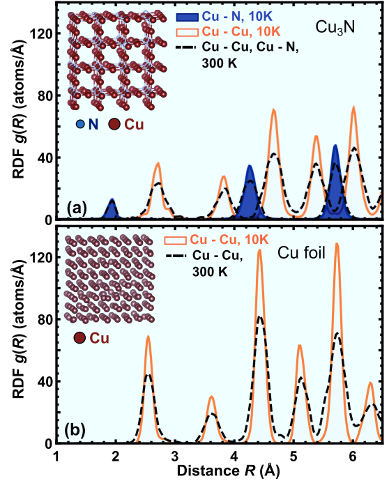
Figure 4: (Color online) Results of RMC/EA simulations for Cu 3 N (a) and for metallic copper (b) at 10 K: the final structure models and partial Cu-Cu and Cu-N radial distribution functions (RDFs). The partial Cu-Cu and Cu-N RDFs at 300 K are also shown for comparison by dashed lines.
