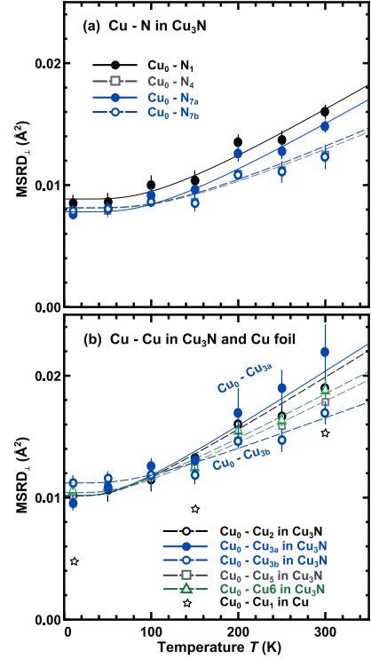
Figure 6: (Color online) Temperature dependencies of the perpendicular MSD factors for Cu-N (a) and Cu-Cu (b) atom pairs in the first seven coordination shells in Cu 3 N. Solid symbols refer to the atom pairs within single -N-Cu-N- chain, while open symbols – to the atoms in the off-chain positions. The data for the nearest neighbours in metallic copper are shown for comparison by open asterisks. Solid and dashed lines are the fits by the correlated Einstein model for atom pairs within single -N-Cu-N- chain and in the off-chain positions, respectively.
