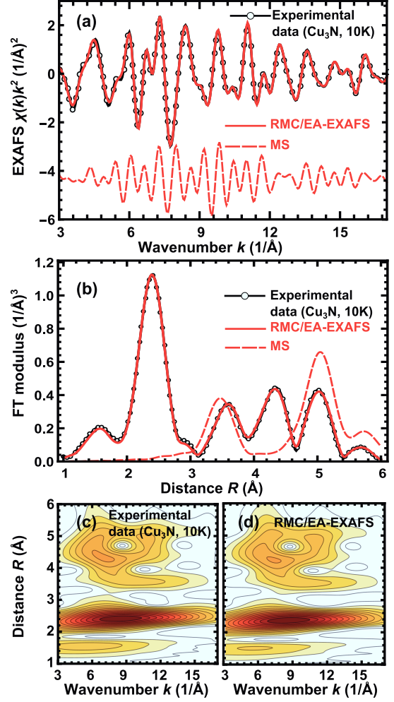
Figure 2: (Color online) Comparison of the experimental ( T = 10 K) and calculated configuration-averaged Cu K-edge EXAFS spectra of \text{Cu}_3\text{N} (a) and their Fourier (b) and Morlet wavelet (c, d) transforms. Dashed lines in panel (a) and (b) show the multiple-scattering contribution to the total calculated EXAFS spectrum and its FT. Spectra in panel (a) are shifted vertically for clarity.
