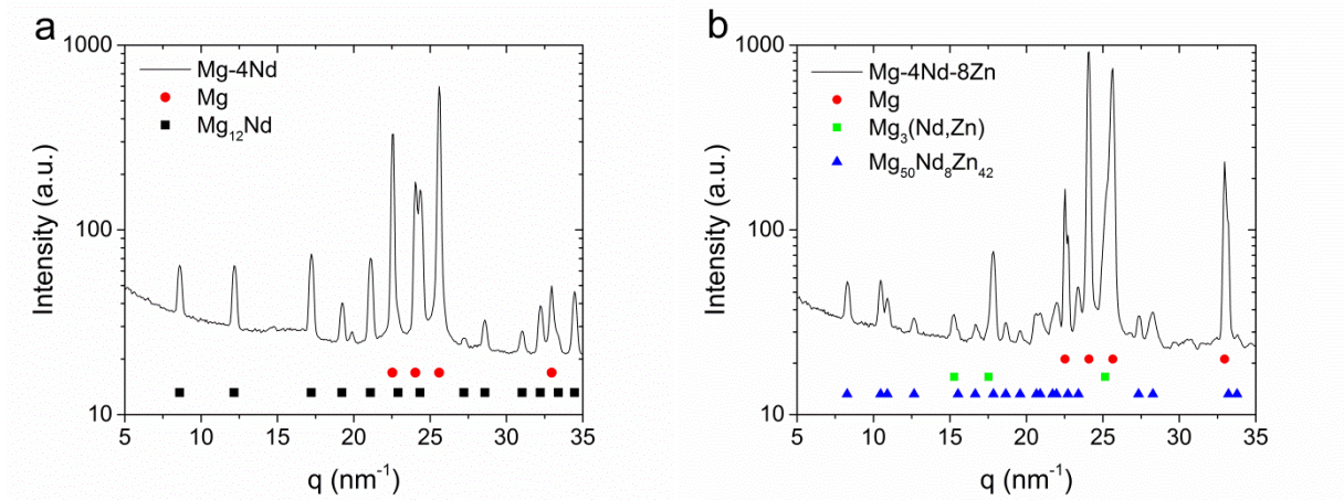
Figure 4: Synchrotron diffraction line profiles for a) Mg-4Nd and b) Mg-4Nd-8Zn.
