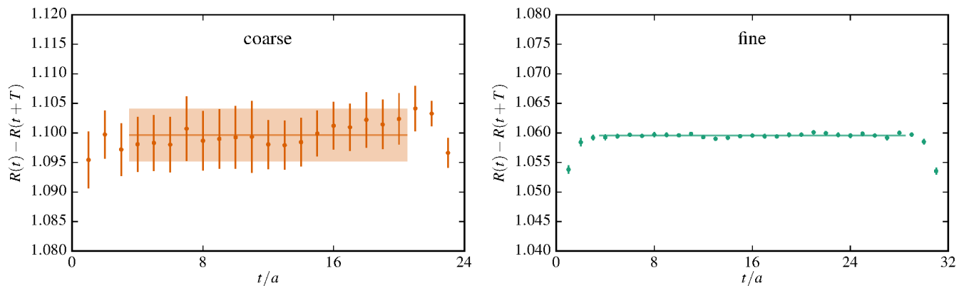
FIG. 8: Determination of Z_V : coarse ensemble (left) and fine ensemble (right). This difference of ratios provides an estimate of Z_V^{-1} .
