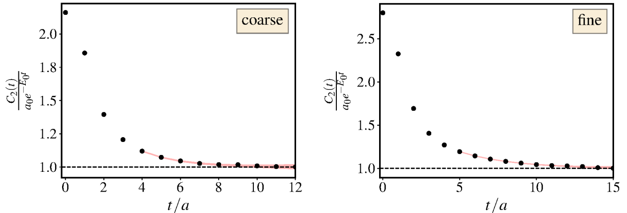
FIG. 2: Plots of the two-point function divided by the ground-state contribution, for both the coarse (left) and the fine (right) ensembles.
