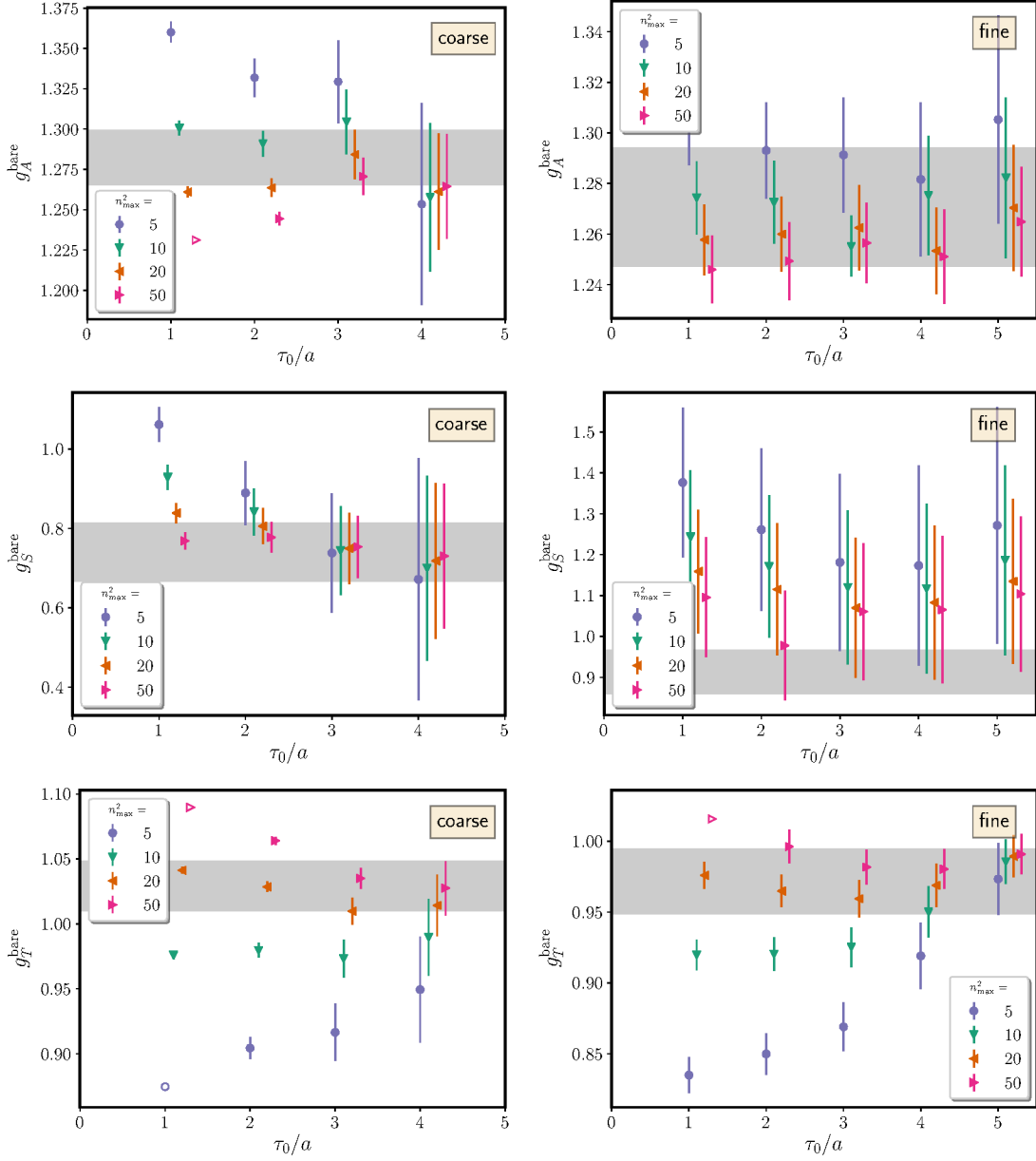
FIG. 12: The bare axial, scalar, and tensor charges obtained using the many-state fit to R^X(\tau, T) for the coarse and fine ensembles. The open symbols refer to fits with p -value < 0.02 . The gray bands denote the final estimates of the charges from Tab. V.
