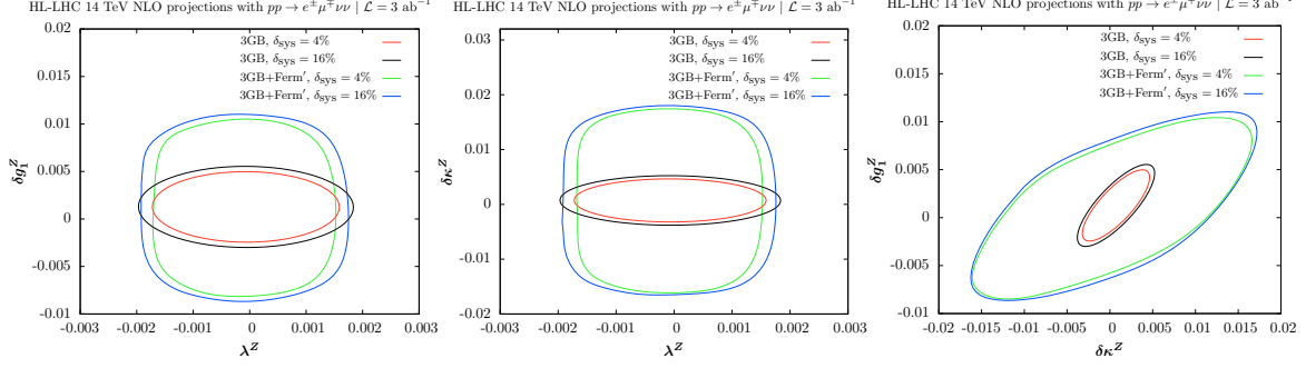
Fig. 40: Projections for 14 TeV with 3 \text{ ab}^{-1} . p_{T,\text{cut}} = 750 \text{ GeV} , corresponding to \delta_{\text{stat}} = 16\% with \delta_{\text{sys}} = 4\% and \delta_{\text{sys}} = 16\% . The curves labelled 3GB have SM Z -fermion couplings, while the curves labelled 3GB +Ferm' allow the Z -fermion couplings to vary around a central value of 0.
