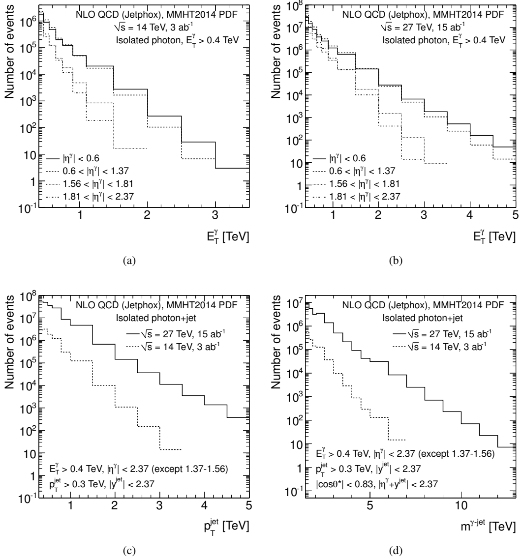
Fig. 55: (a,b) Predicted number of inclusive isolated photon events as a function of E_T^\gamma assuming an integrated luminosity of 3 ab -1 (15 ab -1 ) of pp collision data at \sqrt{s} = 14 TeV (27 TeV) in different ranges of photon pseudorapidity: |\eta^\gamma| < 0.6 (solid histogram), 0.6 < |\eta^\gamma| < 1.37 (dashed histogram), 1.56 < |\eta^\gamma| < 1.81 (dotted histogram) and 1.81 < |\eta^\gamma| < 2.37 (dot-dashed histogram). (c,d) Predicted number of photon+jet events assuming an integrated luminosity of 3 ab -1 (15 ab -1 ) of pp collision data at \sqrt{s} = 14 TeV (27 TeV) as a function of (c) p_T^{\text{jet}} and (d) m^{\gamma\text{-jet}} .
