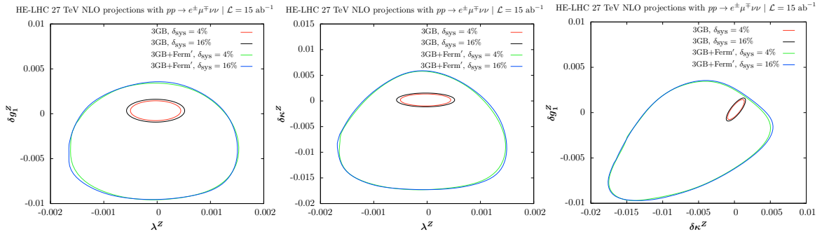
Fig. 41: Projections for 27 TeV with 15 \text{ ab}^{-1} . p_{T,\text{cut}} = 1350 \text{ GeV} , corresponding to \delta_{\text{stat}} = 16\% with \delta_{\text{sys}} = 4\% and \delta_{\text{sys}} = 16\% . The curves labelled 3GB have SM Z -fermion couplings, while the curves labelled 3GB +Ferm' allow the Z -fermion couplings to vary around a central value of 0.
