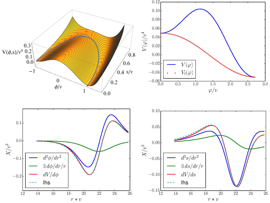
Figure 4: Same as Fig. 2 but for model B.
