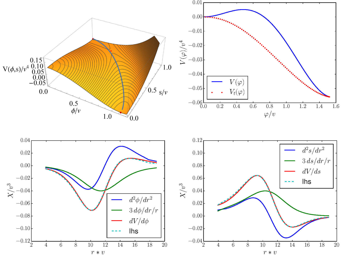
Figure 2: For model A, Upper Left: trajectory in field space of the tunneling solution. Red dots mark the minima and saddle points in V(\phi, s) . Upper Right: potentials V and V_t along the tunneling path, as functions of the canonical field \varphi . Lower Plots: Different contributions to the Euclidean EoM (4) for \phi (left) and s (right). The EoM is fulfilled at the percent level.
