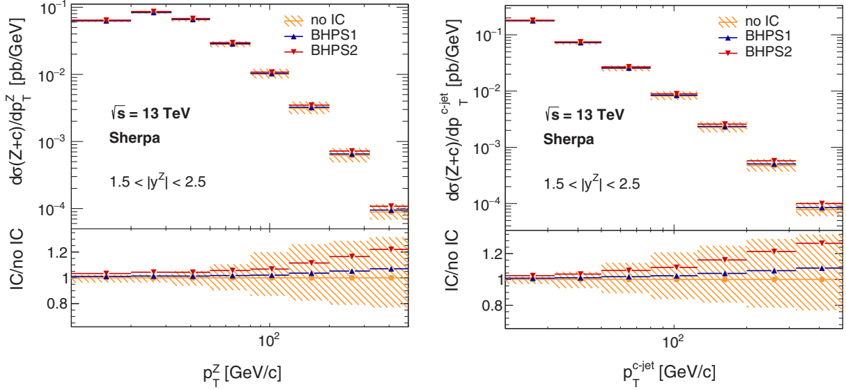
FIG. 3. Predictions for the cross section of Z + c -jet production as a function of the Z boson (left) and c -jet (right) transverse momentum in the forward rapidity region 1.5 < |y^Z| < 2.5 at \sqrt{s} = 13 TeV. The predictions are made with the SHERPA generator using the CT14NNLO PDF with different values for the IC contribution that correspond to BHPS1 and BHPS2 fits and without IC (no IC). The bottom panels show the ratio of predictions for nonzero values of IC to those for no IC. The uncertainty bands represent the uncertainties in the QCD scale (shown only for no IC predictions).
