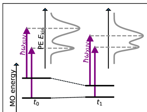
FIG. 3. Schematic description of XUV photoelectron spectroscopy as a probe for chemical shifts. XUV photons with energy \hbar\omega_{XUV} create photoelectrons (PE) with kinetic energies given by the difference of the photon energy and the molecular orbital energy. Ultrafast structural changes induce chemical shifts. 37 From time t_0 (left) to t_1 (right), the molecular orbitals are shifted in energy, which is directly reflected in the photoelectron spectrum.
