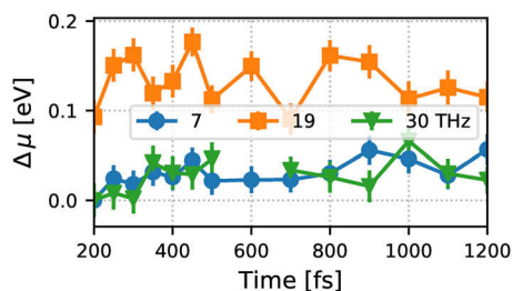
FIG. 7. Time evolution of the 2a_1 peak in the photoelectron spectrum induced by a THz pulse of I = 1 \times 10^{12} W/cm 2 and \nu = 7, 19, and 30 THz. The changes during the pulse duration are omitted for clarity.
