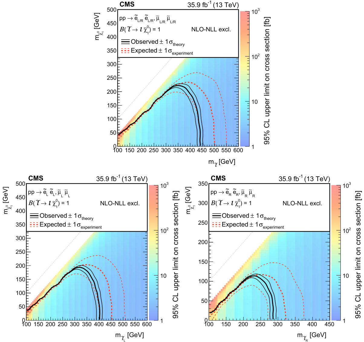
Fig. 5. Cross section upper limit and exclusion contours at 95% CL for direct slepton production of two flavours, selectrons and smuons, as a function of the \tilde{\chi}_1^0 and \tilde{\tau} masses, assuming the production of both left- and right-handed sleptons (upper) or production of only left- (lower left) or right-handed (lower right). The region under the thick red dotted (black solid) line is excluded by the expected (observed) limit. The thin red dotted curves indicate the regions containing 95% of the distribution of limits expected under the background-only hypothesis. The thin solid black curves show the change in the observed limit due to variation of the signal cross sections within their theoretical uncertainties.
