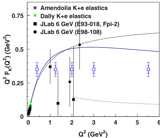
FIG. 3. Kaon form factor from E93-018 and FPI-2 (filled squares) compared to data from Refs. [20,34]. The error bars include the statistical and systematic uncertainty. Also shown are two kaon form factor points (filled circles) we extracted from the cross section data of Ref. [35] using our form factor extraction method. The blue open squares indicate the projected reach and accuracy of data that are anticipated from JLab 12 GeV experiment E12-09-011 [36]. The two error estimates are based on different assumptions about the -t and model dependence of the form factor extractions, with the larger uncertainty being more conservative. The dashed curve shows the monopole using a kaon charge radius of 0.56 fm obtained at low Q^2 in Ref. [20]. The remaining curves are calculations with different kaon parton distribution amplitudes (PDAs). The solid blue line shows the kaon form factor obtained in Ref. [1] using the Dyson-Schwinger equation with rainbow ladder truncation. The curve is consistent within 15% with that obtained using the leading-order (LO), leading-twist (LT) QCD prediction with a pion valence-quark PDA evaluated at a scale appropriate to the experiment. The dotted pink curve corresponds to a LO/LT calculation obtained with the conformal-limit PDA.
