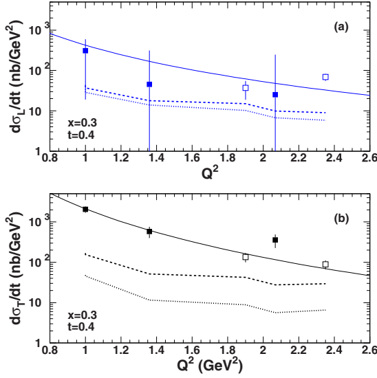
FIG. 4. The Q^2 dependence of the separated cross sections at fixed values of -t = 0.4 (GeV/c) ^2 and x_B = 0.3 . The filled symbols are the scaled cross sections from E93-018 and FPI-2 and the open symbols from E98-108 data. The error bars denote the statistical and systematic uncertainties combined in quadrature. The solid curves show a fit of the form Q^{-n} , for \sigma_L and Q^{-m} for \sigma_T , where n = 5.69 \pm 0.52 and m = 8.47 \pm 0.46 . Calculations using the VR (dashed) and the VGL (dotted) models are also shown.
