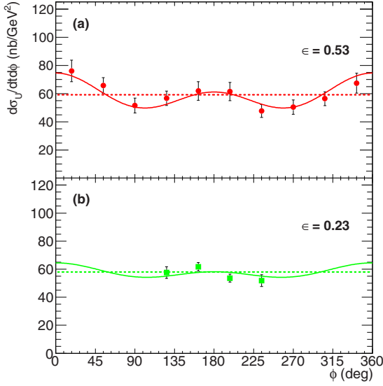
FIG. 2. Unseparated differential cross section extracted in different bins in \phi for the two \epsilon settings of the kinematics with Q^2 = 2.07 \text{ GeV}^2 ( W = 2.31 \text{ GeV} , -t = 0.39 \text{ (GeV/c)}^2 ) of the FPI-2 experiment. The solid lines in panels (a) and (b) are fits to the data using the functional form of Eq. (2). The dashed lines in both panels (a) and (b) indicate the cross section averaged over all \phi bins.
