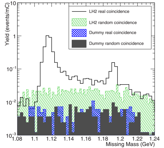
FIG. 1. Missing mass distribution of events within the real (solid line) and random coincidence (green, hatched-shaded area) time window for the FPI-2 setting Q^2 = 2.07 \text{ GeV}^2 and -t = 0.39 (\text{GeV}/c)^2 , integrated over the azimuthal angle. Also shown is the dummy target distribution within the real (blue, cross-shaded area) and random (gray, solid-shaded area) coincidence time window.
