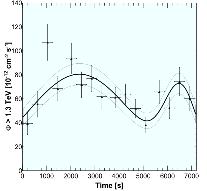
Figure 1. Light curve used for F_s(t) estimation in the range 1.3 < E < 3.25 \text{ TeV} . The thick line corresponds to the best fit and the thin ones correspond to the 1\sigma error envelope. The parameters of the fit function are shown in Table 1.
