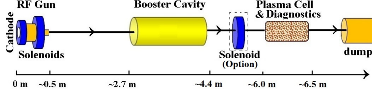
Figure 10: Simulation setup for quasi cw electron beam generation and optimization. The diagram in the dashed frame indicates an option to insert an additional solenoid between the booster cavity and entrance of the plasma cell for further optimization of the transverse beam size. Note that this additional solenoid is currently not yet available but only for design considerations of beam dynamics.
