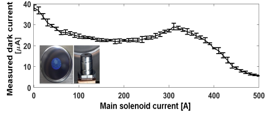
Figure 2: The measured dark current as a function of the main solenoid current for a peak RF power of 6.4 MW in the gun. The inset pictures show the flat cathode and its plug used for these measurements.
