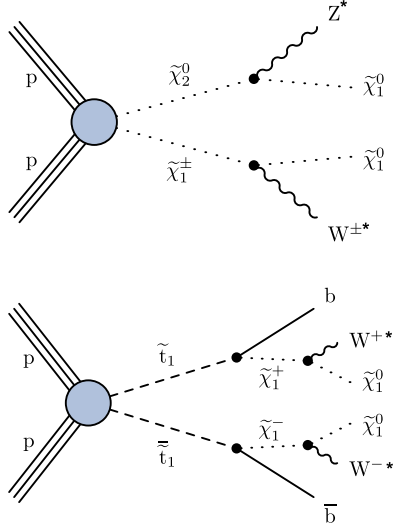
Fig. 1. Production and decay of an electroweakino pair (upper) and of a chargino-mediated \tilde{t}\bar{t} pair (lower).
