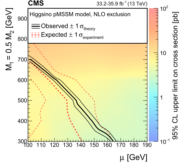
Fig. 7. The observed 95% CL exclusion contours (black curve) assuming the NLO cross sections, with the variations corresponding to the uncertainty in the cross sections for the higgsino pMSSM, which has been introduced in the text. The dashed (red) curves present the band covering 68% of the limits in the absence of signal. The model considers all possible production processes.
