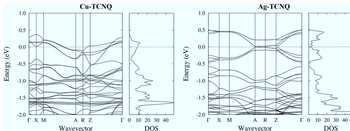
Fig. 7 Detailed band structure and DOS for the bulk CuTCNQ (left panel) and the bulk AgTCNQ (right panel). The bands crossing the Fermi level are visible in the CuTCNQ case. For the AgTCNQ case, there are empty bands close to the Fermi level separated from the filled bands by a micro-gap in which is located the Fermi level. The density of states has been convoluted with a Gaussian of a width of 0.025 eV (one order of magnitude narrower than that used in the DOS presented in Fig. 6).
