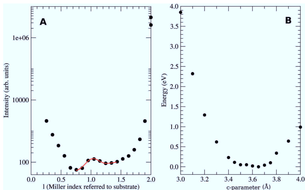
Fig. 4 (A) Specular X-ray diffraction 00 l crystal ROD intensity. The l Miller index is referred to perpendicular to the substrate surface lattice Cu(001) (with c = 3.615 Å); (B) calculated total energy of the CuTCNQ versus its c parameter.
