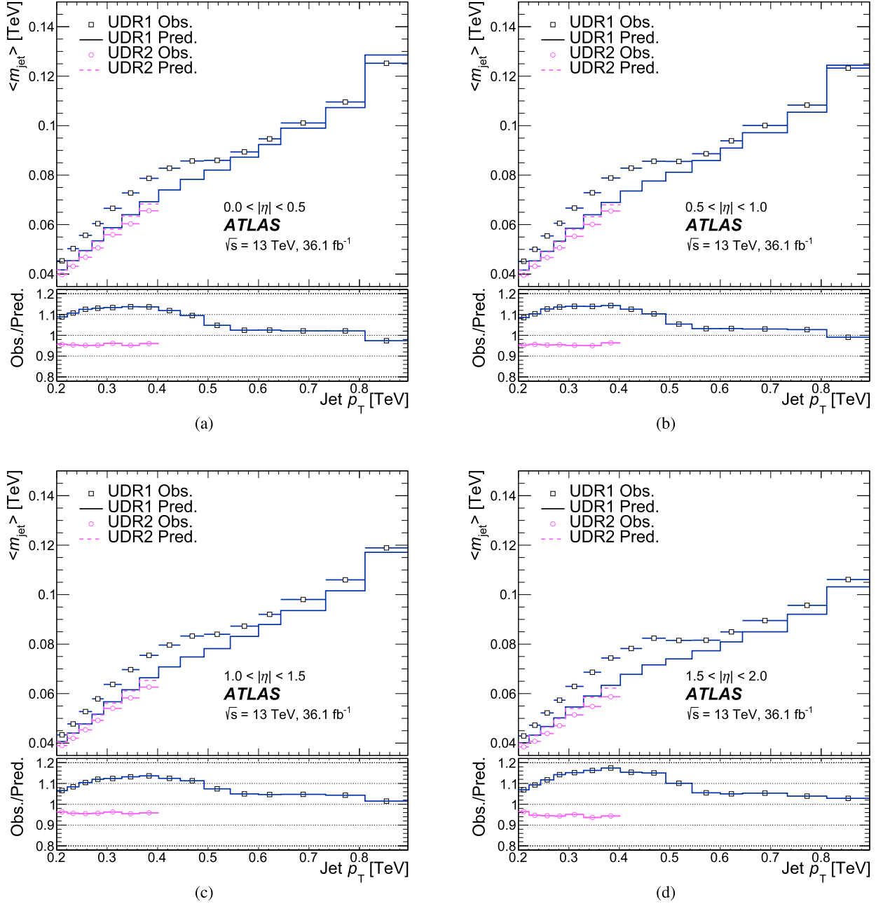
Fig. 4. The average observed and predicted jet masses (top panes) and the jet mass responses (bottom pane) in UDR1 and UDR2 are shown for four different pseudorapidity regions.
