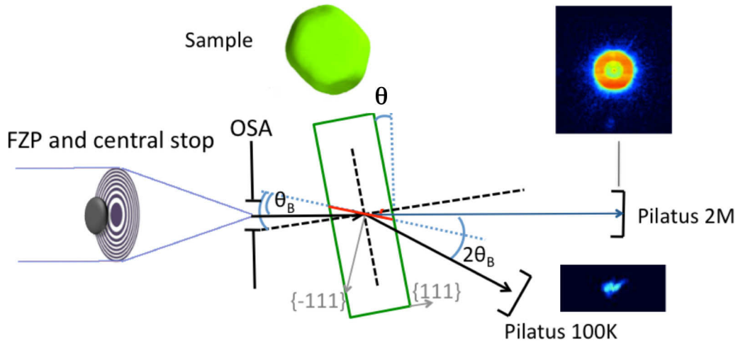
FIG. 1. Setup schematic. A Fresnel zone plate is used to focus the beam. The Au nanocrystals were placed at the focus with their \bar{1}11 crystal planes oriented at the angle \theta_B with respect to the incoming beam. A 2D detector is placed in the forward direction and another 2D detector in the direction of the Bragg reflection.
