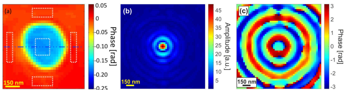
FIG. 2. (a) Reconstructed phase image of a nanocrystal at an angle close to the \bar{1}11 Bragg reflection. The regions marked with dotted and dashed lines were used for quantitative analysis (see text for details). (b) Reconstructed amplitude of the illumination probe, showing a focused beam of 110-nm size. (c) Reconstructed phase of the illumination probe.
