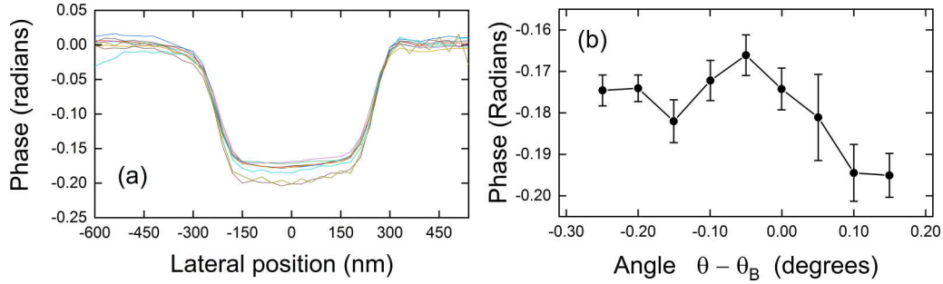
FIG. 3. (a) Phase profiles along the dashed-dotted line in Fig. 2(a) for different angles \theta around the Bragg reflection. (b) Phase-shift difference between the particle and the outside region as a function of the Bragg angle, \theta .
