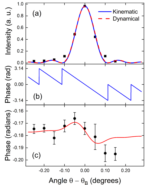
FIG. 5. (a) Rocking curve of diffracted intensity points with kinematical fitting curves from Eq. (1) shown as a blue line and the dynamical calculation as a red line. (b) Corresponding phase of the diffracted intensity in Eq. (1). (c) Measured transmitted phase shift, identical data to those shown in Fig. 3(b), together with the dynamical curve, calculated from Eq. (3) by the method of Gorobtsov and Vartanyants [36].
