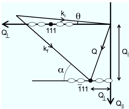
FIG. 4. Reciprocal space construction of the perpendicular component of momentum transfer needed to calculate the sample reflectivity profile. The orientation is the same as the experimental schematic layout in Fig. 1. The thickness fringes of the sample slab, perpendicular to the surface, are shown schematically as ellipses.
