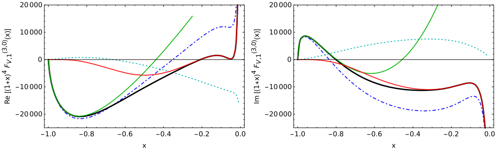
Fig. 4. The O(\epsilon^0) contribution to the vector three-loop form factors \text{Re}[F_{V,1}^{(3)}] (left) and \text{Im}[F_{V,1}^{(3)}] (right) as a function of x \in [-1, 0] . Full red line: expansion around x = 0 ; Full green line: expansion around x = -1 ; Dotted line: n_l -contributions. Dash-dotted line: leading color contribution of the non-singlet form factor; Full black line: sum of the complete non-singlet n_l -contributions for n_l = 5 and the color-planar non-singlet form factor.
