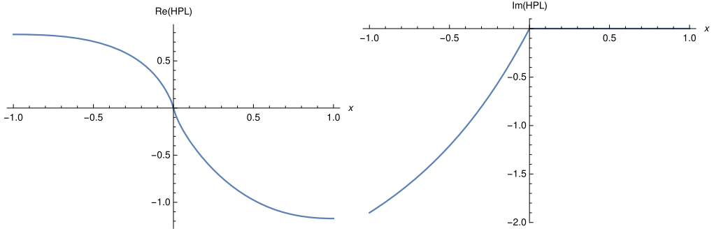
Fig. 6. The real (left panel) and imaginary part (right panel) of the function H[\{6, 0\}, 0, x] in the region x \in [-1, 1] .
