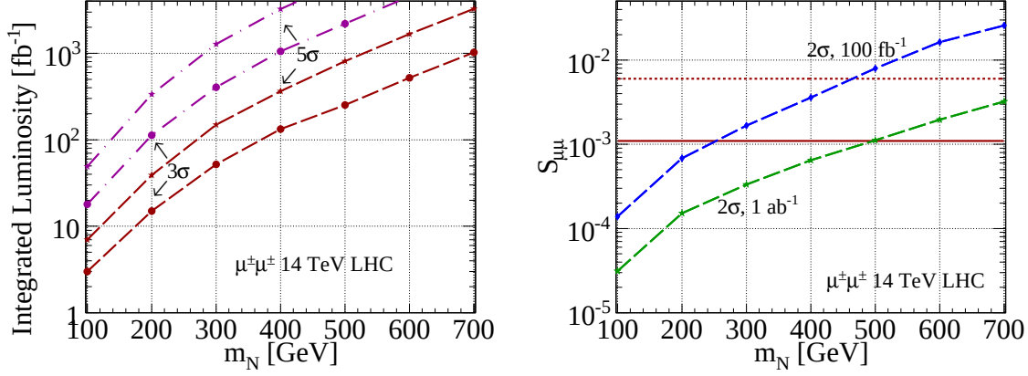
Fig. 76: Left: required luminosity for 3 (5) \sigma evidence (discovery) using the LNV final state \mu^\pm\mu^\pm jj , as a function of the heavy neutrino mass, m_N , assuming optimistic (brown) and pessimistic (purple) mixing scenarios [1440]. Right: sensitivity to N - \mu mixing [1440] with the optimistic (pessimistic) mixing scenario is given by the horizontal dashed (full) line.
