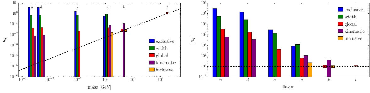
Fig. 63: Summary of the HL-LHC projections discussed in the main text: from exclusive decays (blue), from Higgs kinematic distributions (purple) and from inclusive constraints (yellow), compared to the present 8 TeV constraints from the h \rightarrow \gamma\gamma and ZZ line shapes (green), and from global fits (red).
