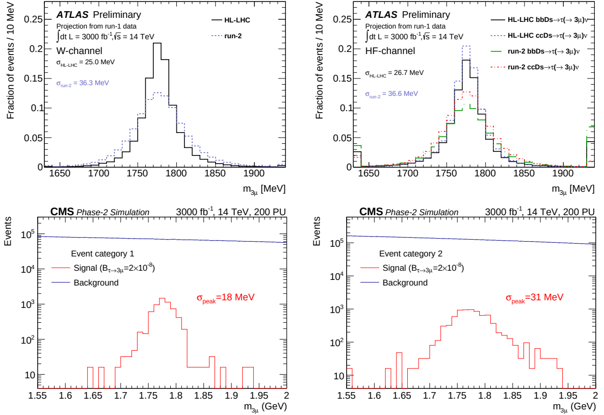
Fig. 36: (Top) Comparison of ATLAS tau mass resolutions in the W - (left) and HF-channels (right) in Run-2 and under HL-LHC detector conditions. Widths are estimated from a double-Gaussian fit. (Bottom) CMS trimuon invariant mass m_{3\mu} for the \tau \rightarrow 3\mu signal (red) and background (blue) after all event selection cuts, for Category 1 (left) and Category 2 (right) events, as defined in the text. The signal is shown for \mathcal{B}(\tau \rightarrow 3\mu) = 2 \times 10^{-8} . CMS results refer to the HF channel; plots are taken from [435].
