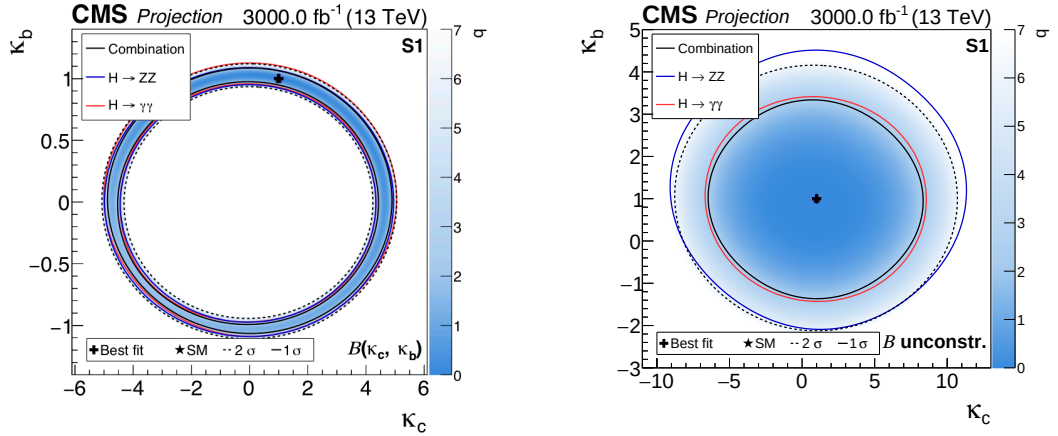
Fig. 69: Left: projected simultaneous fit of \kappa_b and \kappa_c from 3ab ^{-1} 13 TeV data, assuming current systematics (Scenario 1). The one standard deviation contours are drawn for the h \rightarrow \gamma\gamma channel (the h \rightarrow ZZ , the combination of h \rightarrow \gamma\gamma and h \rightarrow ZZ ) with solid red (blue, black). For the combination the two standard deviation contour is drawn as a black dashed line. The negative log-likelihood value are given on the coloured axis. Right: same as left, but with the branching fractions implemented as nuisance parameters with no prior constraint. (Taken from [1354].).
