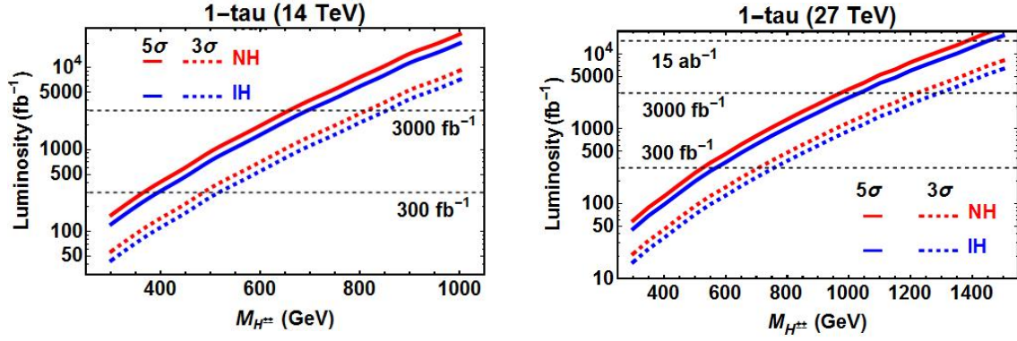
Fig. 78: Requisite luminosity for 5(3)\sigma discovery (evidence) as a function of M_{H^{\pm\pm}} for the process pp \rightarrow H^{++}H^{--} \rightarrow \tau_h \ell^\pm \ell^\mp \ell^\pm \ell^\mp , where \tau^\pm \rightarrow \pi^\pm \nu , for the NH and IH at \sqrt{s} = 14, 27 TeV.
