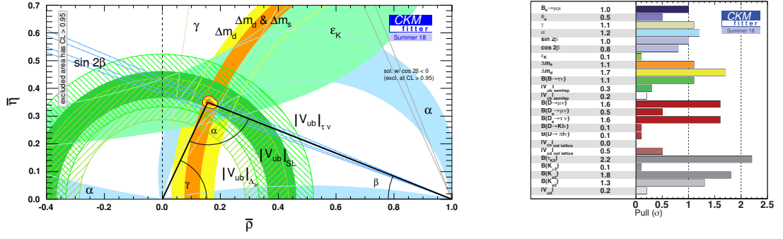
Fig. 4: Results for the CKMfitter global fit of the CKM parameters as of Summer 2018. See Ref. [37] for more detail.
