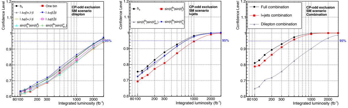
Fig. 71: Expected CL, assuming the SM, for exclusion of the pure CP -odd scenario, \kappa_t = 0 , \tilde{\kappa}_t = 1 , as a function of the integrated luminosity. Left: using the t\bar{t}h ( h \rightarrow b\bar{b} ) dileptonic analysis only, middle: using the t\bar{t}h ( h \rightarrow b\bar{b} ) semileptonic analysis only, right: combining observables in each individual channel and combining both channels, treating the observables as uncorrelated. A likelihood ratio computed from the binned distribution of the corresponding discriminant observable was used as test statistic.
