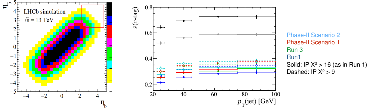
Fig. 65: Left: 2D histogram showing the coverage of the LHCb acceptance for the b\bar{b} pair produced by the Higgs decay in associated production with a W or a Z boson. Right: LHCb c -jet SV-tagging efficiency for different scenarios in the HL-LHC conditions.
