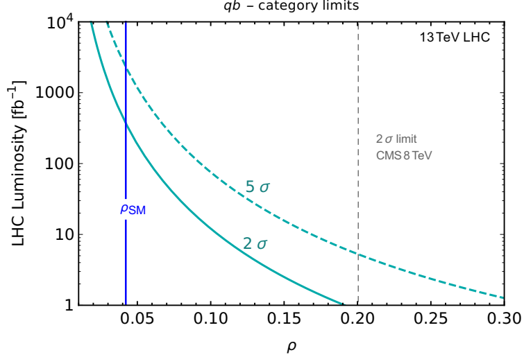
Fig. 62: Illustration of statistical limits on the ratio \rho \simeq (|V_{ts}|^2 + |V_{td}|^2)^{1/2}/|V_{tb}| from an analysis of Cabbibo-suppressed top decays in leptonic t\bar{t} events at 13TeV LHC. See text for details.
