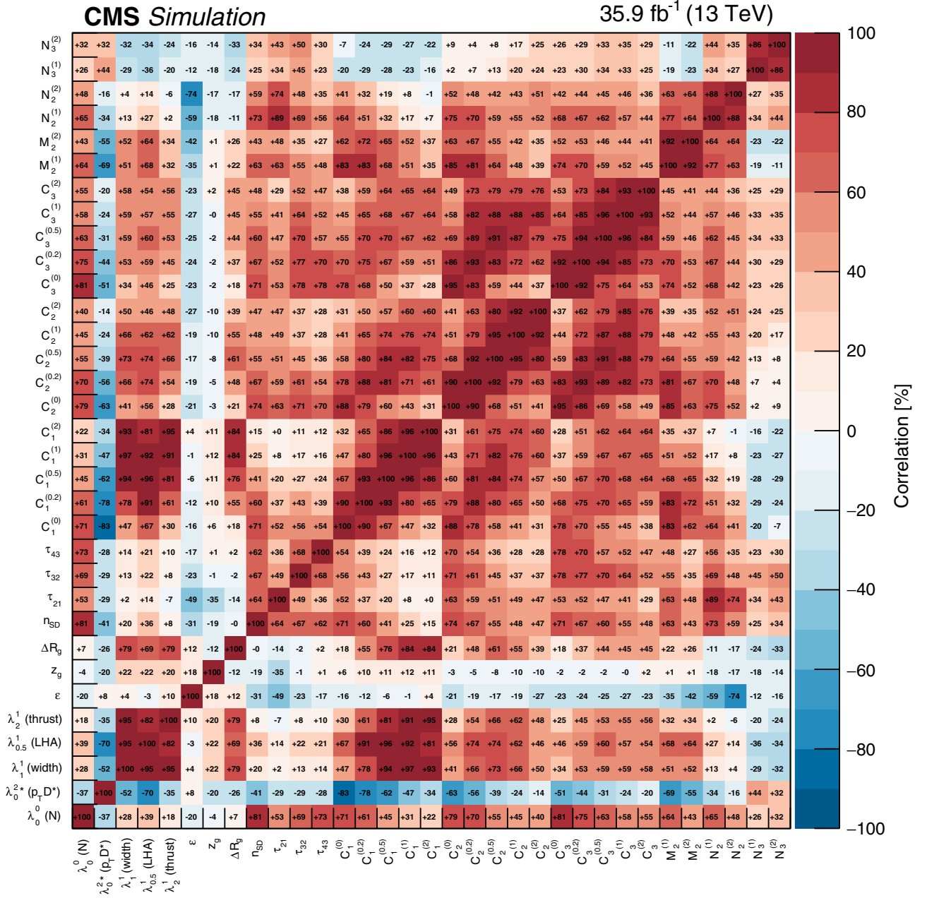
FIG. 20. Correlations of the jet substructure observables used in this analysis obtained at the particle level.
