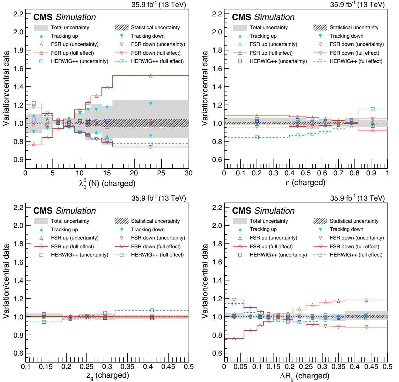
FIG. 3. Systematic uncertainties for the charged multiplicity \lambda_0^0(N) (upper left), jet eccentricity \epsilon (upper right), groomed momentum fraction z_g (lower left), and angle between the groomed subjects \Delta R_g (lower right). The uncertainties from FSR and HERWIG (open markers) are compared to the full effect of these variations at the particle level (open markers with lines).
