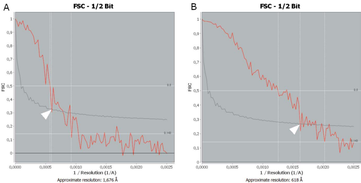
Figure 9 Estimation of the 3D-resolution via FSC sequential comparison, defined by the half-period of the spatial frequency of reconstructed slices. (A) Original (167.6 nm) and (B) after rapid alignment of the projections (61.8 nm), as indicated by the arrow heads.
