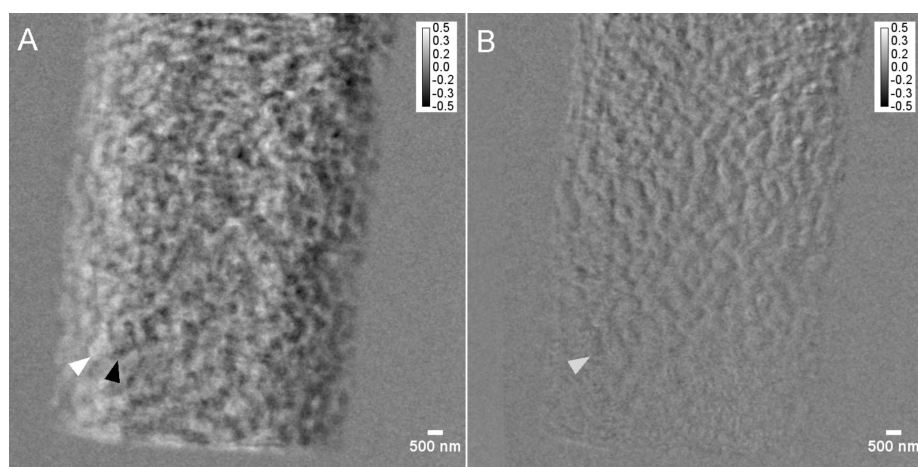
Figure 3 Flat-field-corrected projections of a projection acquired at 0° subtracted with a projection acquired at 180° (after horizontal flipping). (A) Original misplacement of sample and (B) after correction of the sample movement via rapid alignment and forward projecting (number of iterations: 40), which severely reduces the sample-movement error seen in (A), especially at the top of the sample (displayed as upside-down in XRM mode). The images are displayed on a 32-bit grey-level scale. Similar features have been marked with arrow heads. (Note that the correction of the projections worked better on the top of the sample than on the bottom part, which is most likely related to a slight wobble or tilt of the rotation axis, which could not be 'entirely' corrected for by the rapid alignment algorithm.)
