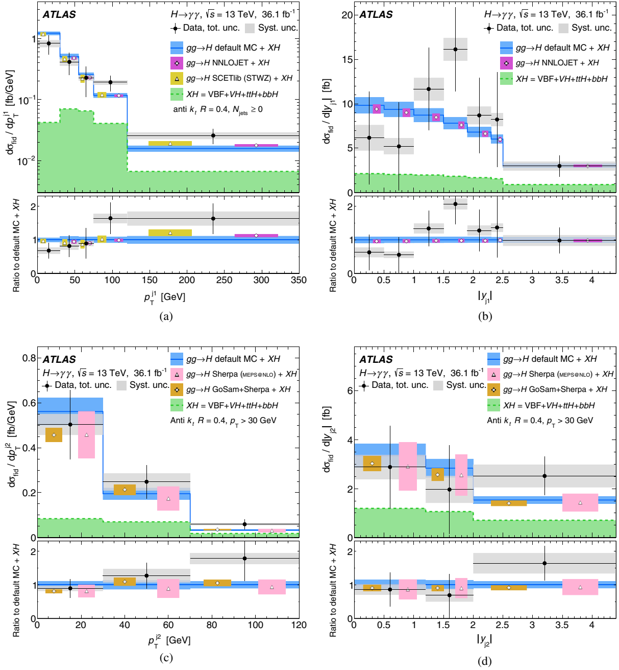
FIG. 27. The differential cross sections for pp \rightarrow H \rightarrow \gamma\gamma as a function of (a) p_T^{j_1} , (b) |y_{j_1}| , (c) p_T^{j_2} , and (d) |y_{j_2}| are shown and compared to the SM expectations. The data and theoretical predictions are presented in the same way as in Fig. 26. In addition, the NNLOJET and SCETLIB(STWZ) predictions, the NNLOJET prediction, and the SHERPA (MEPS@NLO) and GoSAM predictions, described in the text, are displayed in (a), (b) and (c+d), respectively.
