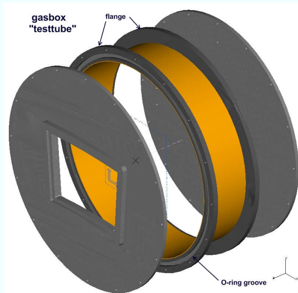
Figure 8.4: 3-Dimensional representation of the gas container and mechanical support structure of the SM-TPC.
