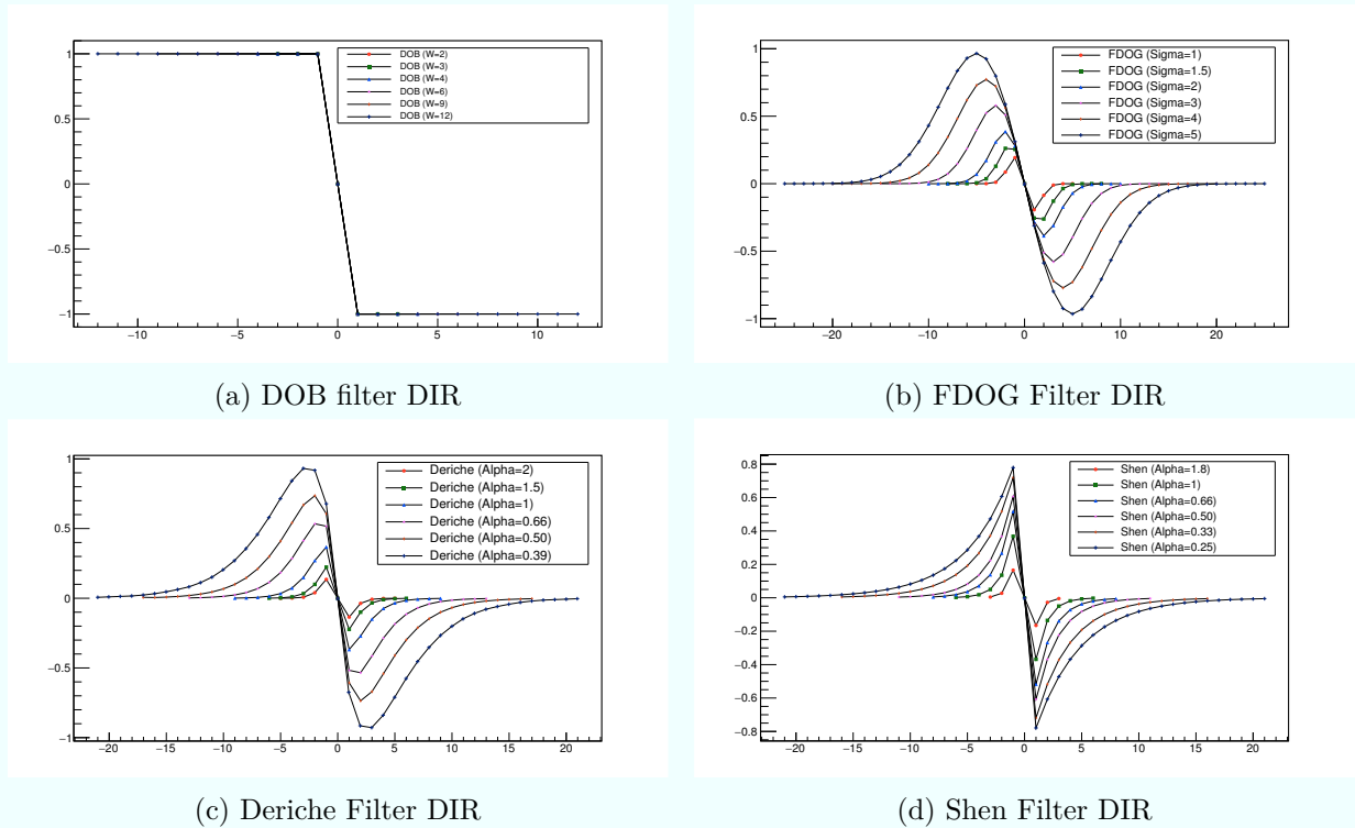
Figure 11.1: Impulse response of different convolution filters. For each of them we plot this function for different values of the characterizing parameter.
