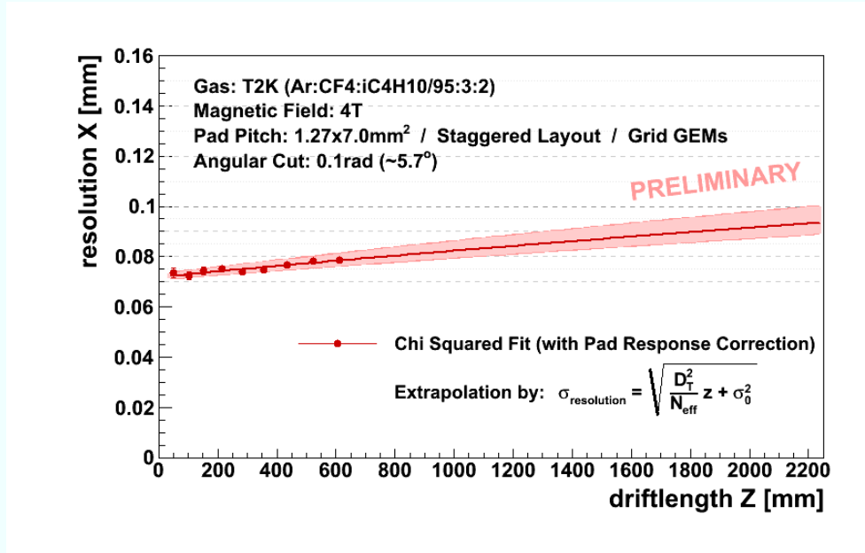
Figure 7.11: Point resolution of a GEM based medium size prototype in a 4T magnetic field. The resolution beyond \approx 600 mm could not be measured directly due to the limited length of the detector and is estimated using the formula visible in the lower right corner.
