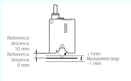
(a) Sketch of the configuration of the LK-G10 Laser displacement sensor installed to perform a profile measurement.
