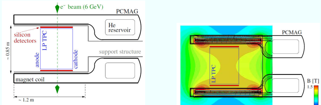
(a) Scheme of the position of the magnet and the detector relative to the beam incoming from the DESY II T24 beam line.
