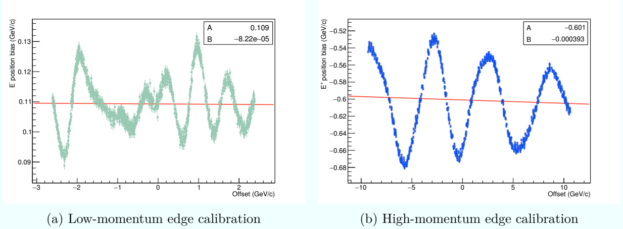
Figure 12.34: Calibration graphs of the high- and low-momentum edge measurements. Each data point corresponds to a measurement of the localization parameters on a different distribution template obtained by applying a random offset to the signal sample. Superimposed to the measurement set we displayed a first degree polynomial fit to the data showing a long range independence of the bias from the offset.
