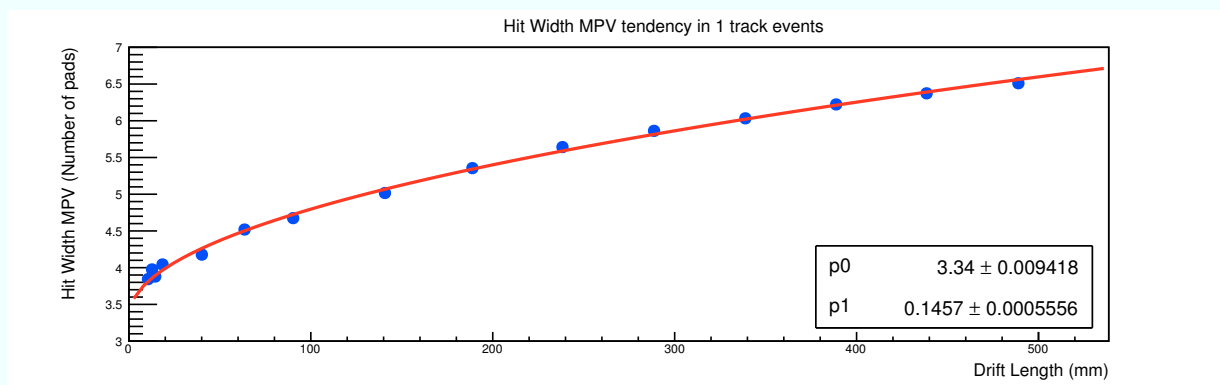
Figure 9.34: Most probable value of the hit width at different drift lengths. Each data point is obtained from the MPV of a Landau function fit to the hit width distribution recorded for a single test-beam run. The error bar, smaller than the marker, is the statistical error on the determination of the MPV from the fit. The algorithm to select the hits is described in the text. The points were fit with the following function: p_0 + p_1\sqrt{x}
