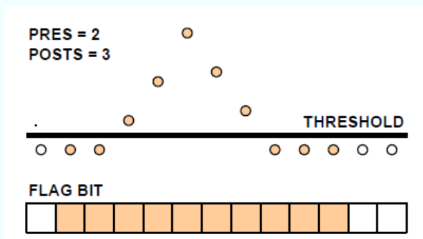
Figure 6.10: Sketch of the zero suppression processing step of the ALTRO chip (from [98]). Each digital sample is represented by a small circle and those colored are saved in the chip memory. In this case all of those over the threshold value and 2 additional samples before the first one over threshold and 3 in the tail are saved.
