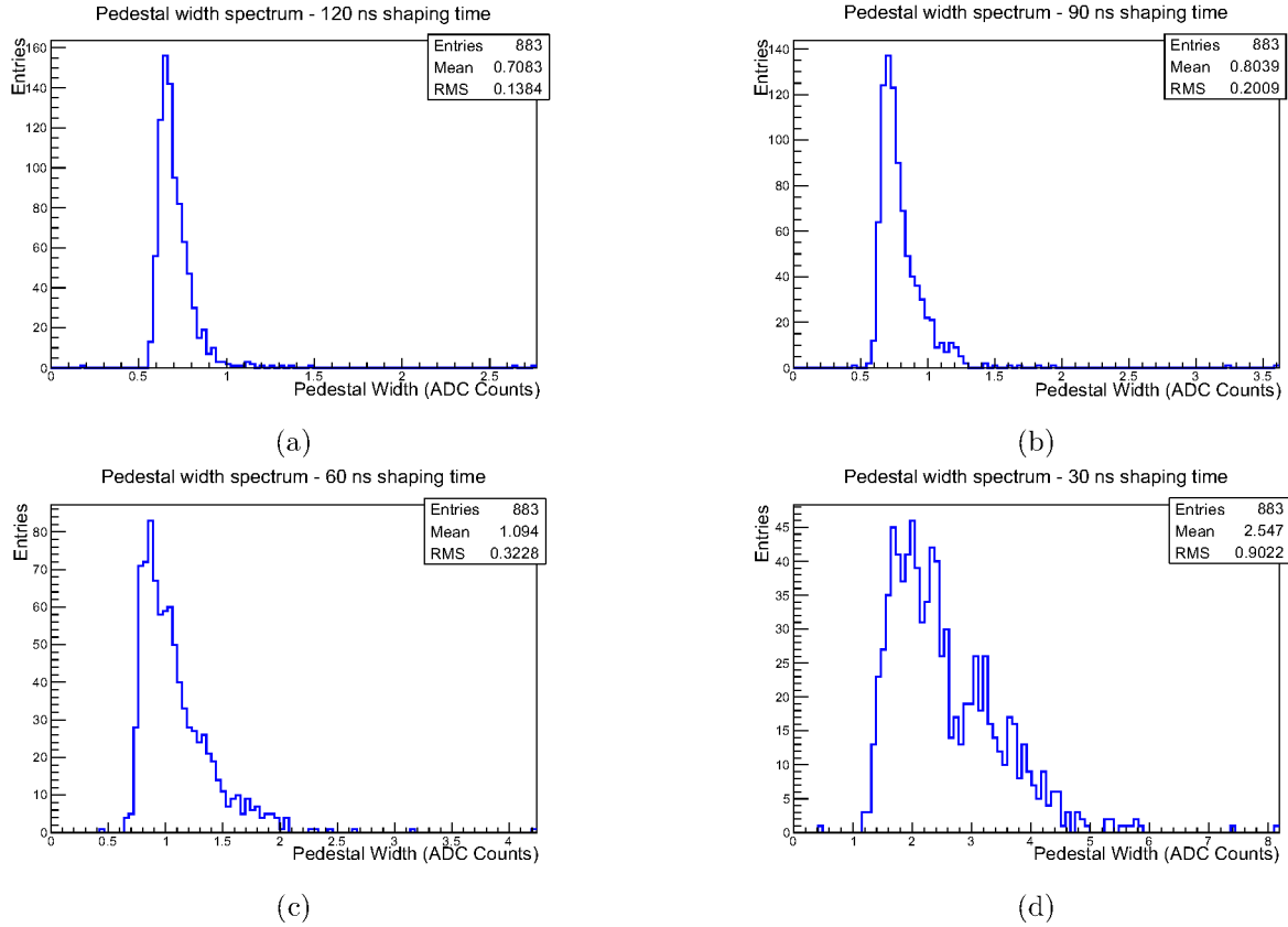
Figure 9.10: Comparison of the pedestal width spectra for runs recorded with different electronics shaping times. The other settings of the readout system were kept to the nominal values listed in tab. 8.5.
