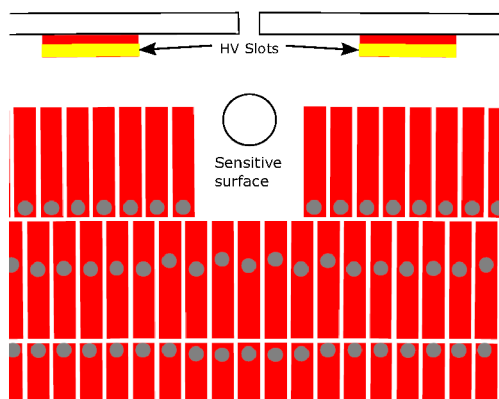
Figure 7.7: Drawing of the central area of the top border of the readout board. It shows the HV slots separated from the readout pad by a gap large enough to fit a ceramic component. It is also visible, in the center of the sketch, the through hole used to fix the S^3 system to the back-frame.
