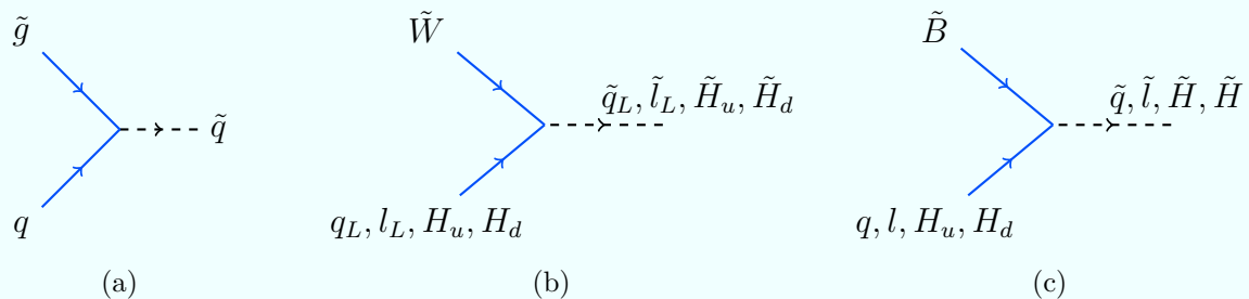
Figure 1.2: Additional matter-gauge couplings introduced in the supersymmetric extensions of the standard model. In (a) the coloured coupling and in (b) and (c) the electro-weak couplings. For each of the represented diagrams there is another one with the corresponding anti-particles.
