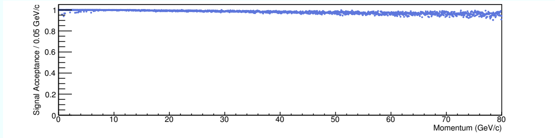
(b) Charged energy ratio acceptance as a function of J_L momentum
