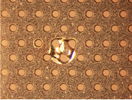
Figure 5.2: Microscopic photo of the surface of a GEM foil. The hexagonal pattern of the holes on the GEM surface is clearly visible. At the center of the photo is also visible the damage to the foil surface produced by a powerful discharge.
