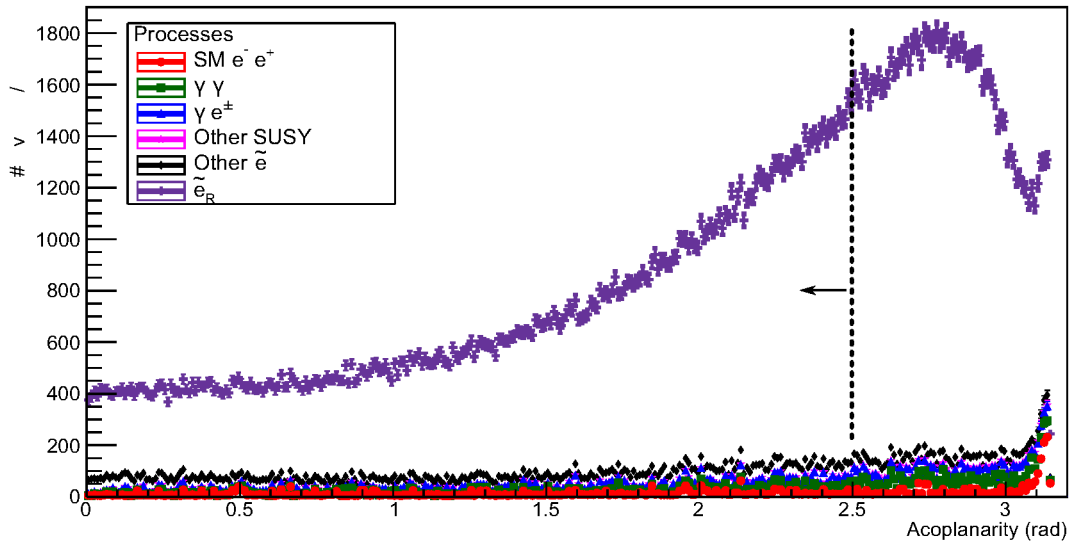
Figure 12.28: The distribution of the Acoplanarity variable values for all the process categories after the application of the Missing P_T cut. The histograms are stacked on top of each other. The dashed black line represents the threshold of the cut applied to this variable.
