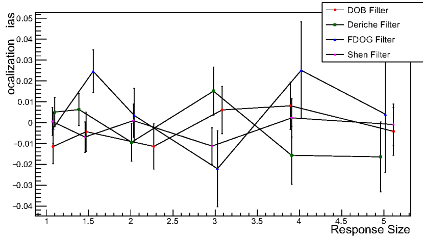
Figure 11.5: The localization bias of all the filter under evaluation is plotted against the filter size. The value is generally compatible with 0 at all sizes. The parameter is calculated for an ideal filter with S/N = 0.5
