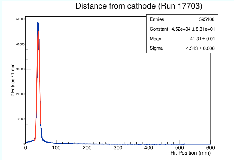
Figure 9.18: Distribution of the hit coordinate along the drift direction for a test-beam run. The peak of the distribution was fit with a Gaussian function to measure the beam position and width.
