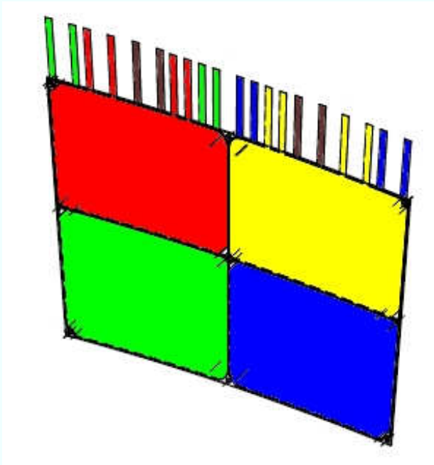
Figure 7.4: Sketch of the layout of the sectioned side of the GEM showing in different colour each sector and the group of electrodes connected to that sector. The 4 black electrodes are those connected to the back side of the GEM.
