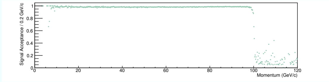
(a) Charged energy ratio acceptance as a function of J_H momentum
