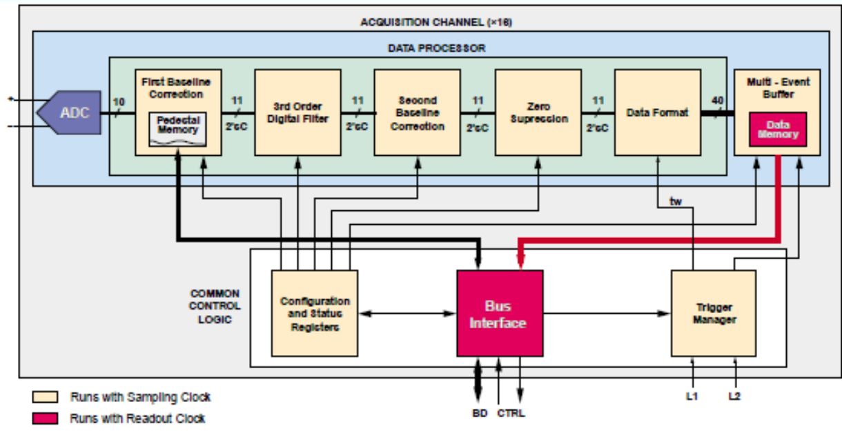
Figure 6.9: Details of the processing of the digital signals performed by the ALTRO chip for each of 16 readout channels (from [98])
