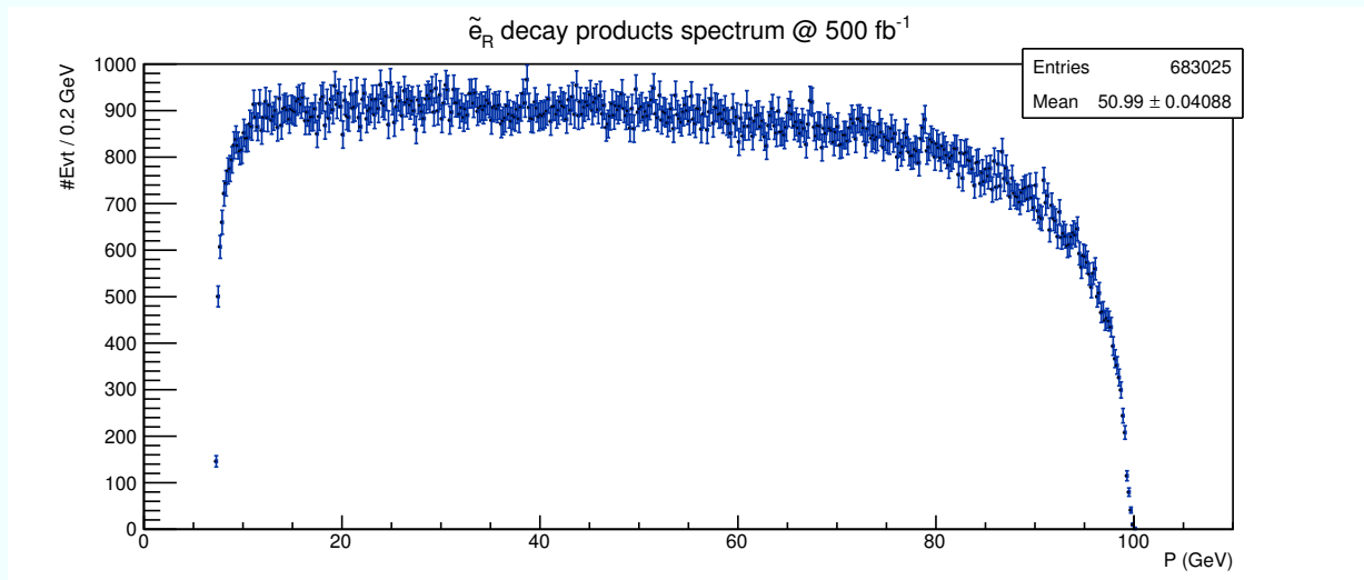
Figure 10.3: Momentum distribution of the electron and positrons produced by the decay of a \tilde{e}_R pair, generated using a realistic beam energy distribution. The masses and cross-section are calculated with the tools described in § 12.1. The momentum is directly extracted from the generator files, before any detector reconstruction is applied. The amount of simulated data corresponds to 500 fb -1 at 500 GeV with a 80% right-polarized electrons and 30% left-polarized positrons
