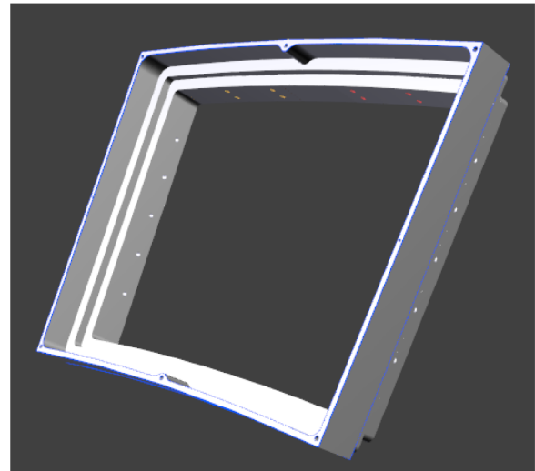
Figure 7.3: 3-dimensional rendering of the GridGEM module back-frame as seen from the drift side. It can be noted the presence of the 6 screw-holes on the corners and in the middle of the two arcs and the 2 small dowel holes in the middle of the side walls.
