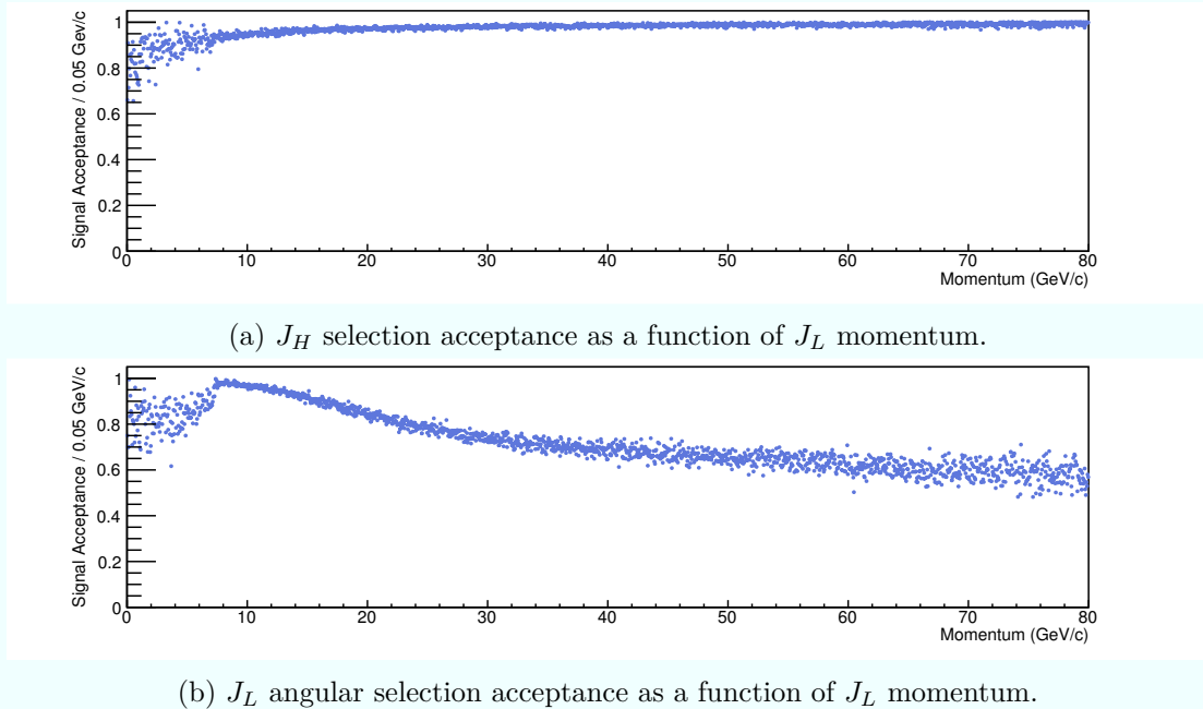
Figure 12.24: The signal acceptance of the J_H and J_L angular selections plotted as a function of the J_L momentum in the signal sample.
