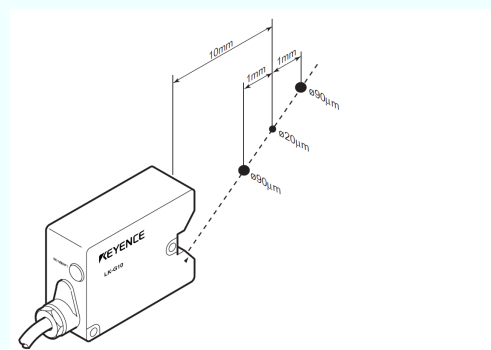
(b) Sketch of the laser beam spot produced by the LK-G10 displacement sensor on a target surface at different distances from the measuring head.
