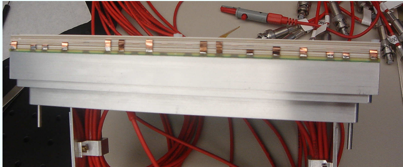
Figure 7.14: Top arc of the GridGEM module at the end of the installation procedure showing the electrodes coming from the different layers in the GEM stack soldered to the readout board.
