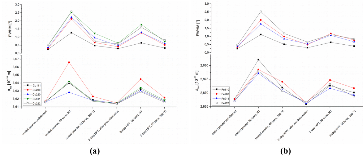
Figure A5: Peak width (full width at half maximum, FWHM) and lattice parameter calculated from the XRD peak positions, a_{hkl} , for the (a) Cu and (b) Fe phases.
