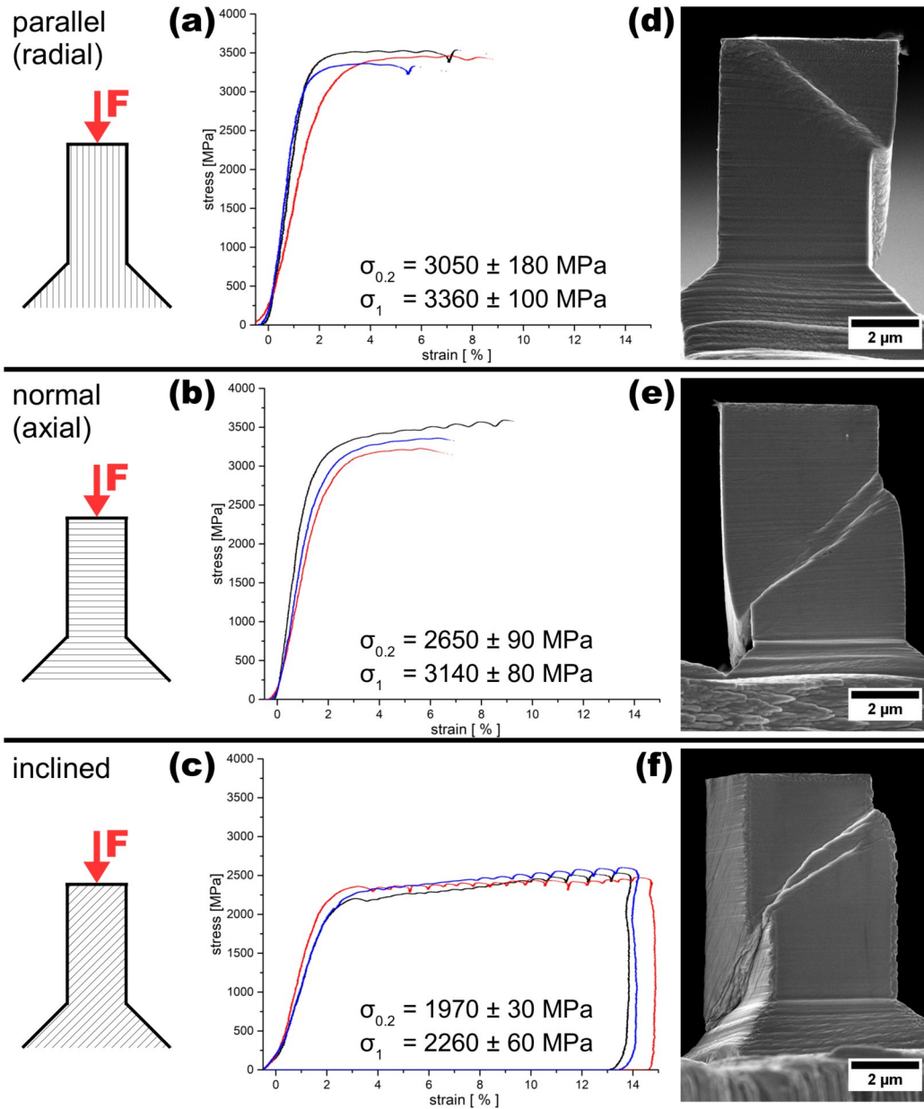
Figure B6: Engineering stress-strain curves from micropillar compression of HPT-deformed martensite (1 turn, r = 3\text{ mm} , \varepsilon_{vM} = 15 ) tested in (a) parallel, (b) normal and (c) inclined loading direction. The three curves in each graph correspond to three different micropillars tested in each direction and the yield stresses at 0.2 % and 1 % plastic strain, \sigma_{0.2} and \sigma_1 , are given as the average value with the standard deviation from the three samples each. Corresponding exemplary post-mortem SEM images for the three orientations are shown in (d-f).
