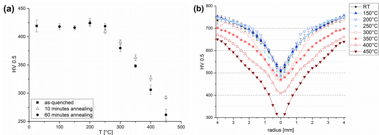
Figure C3: (a) Microhardness of as-quenched martensite after isothermal tempering. (b) Microhardness profiles after isothermal tempering for 60 minutes and subsequent HPT at room temperature (1 revolution).
