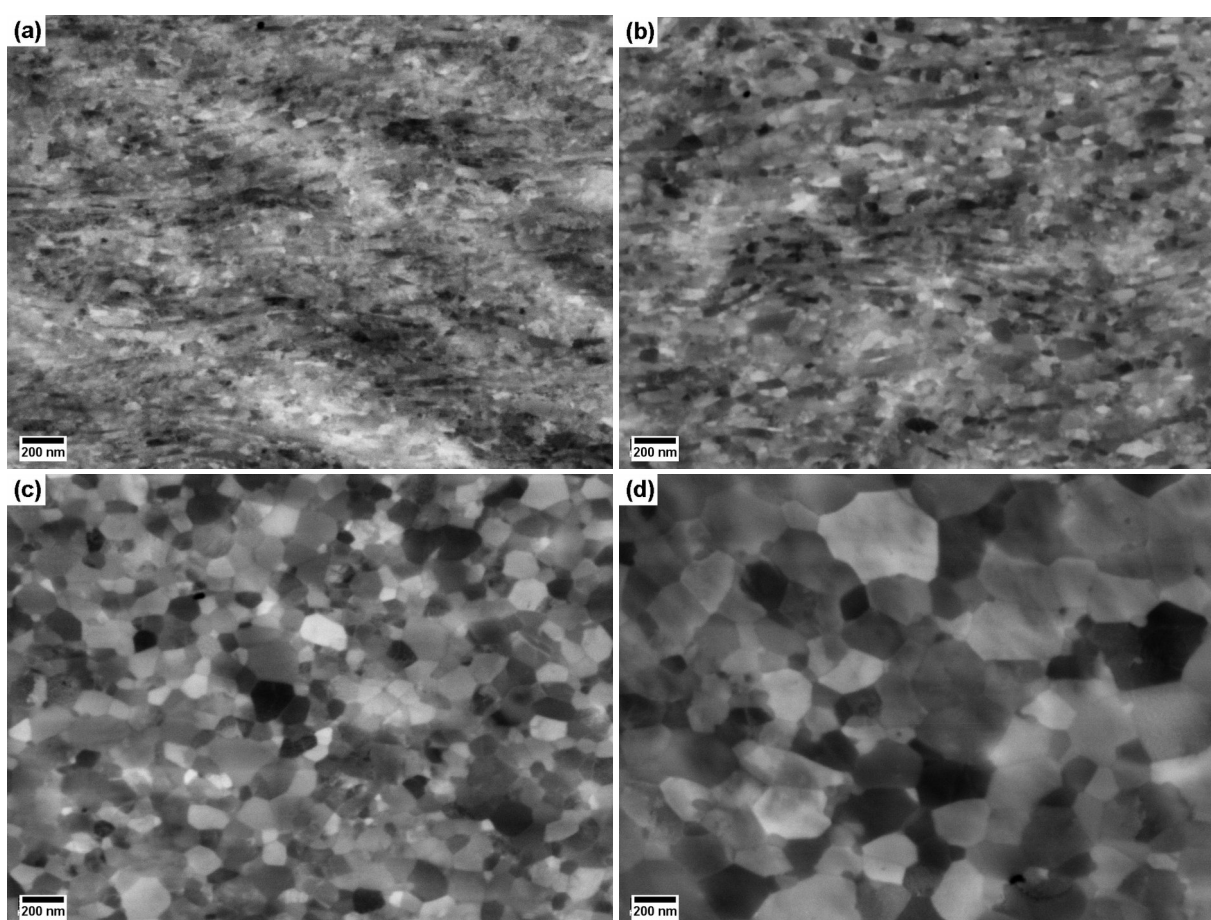
Figure C6: Microstructures after annealing of HPT-treated martensite for 60 minutes at (a) 200 °C, (b) 350 °C, (c) 400 °C and (d) 450 °C ( r = 3 mm, 1 revolution, \varepsilon_{VM} = 15 ).
