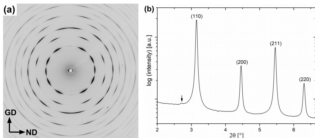
Figure D3: (a) High-energy XRD pattern of a B50 sample recorded with the primary beam in-plane. GD and ND indicate the growth direction and the in-plane direction, respectively. (b) Diffractogram obtained from (a) via integration over all azimuthal angles. The only indication of a small peak besides the ferritic phase is marked with an arrow.
