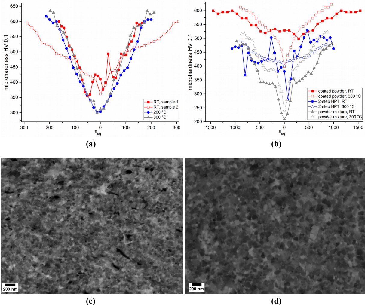
Figure A4: The effect of elevated temperature on the structure and hardness evolution: (a) Hardness profiles of HPT samples from coated powder after 10 turns at different temperatures (the differences between the two room-temperature samples can be attributed to different amounts of cracking, cf. Figure A3b); (b) Hardness profiles of HPT samples after 50 turns; Back-scattered electron micrographs of (c) coated powder and (d) pre-deformed (two-step HPT) powder mixture after 50 turns at 300 °C, measured at a radius of 3 mm ( \epsilon_{eq} = 700 without previous deformation).
