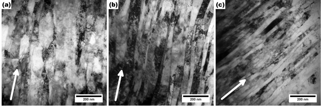
Figure B2: TEM micrographs of a sample after one turn HPT. (a) and (b) are taken at a radius of r = 1 mm ( \varepsilon_{VM} = 5 ) whereas (c) is from the same sample at r = 3 mm ( \varepsilon_{VM} = 15 ). The white arrows indicate the shear direction.
