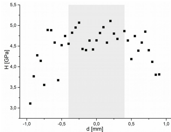
Figure 6: Hardness profile over the height of a as-quenched martensitic Ck10 sample as obtained from nanoindentation with a cube corner indenter with a maximum load of 6 mN. The gray area indicates the approximate region that was used for HPT deformation after grinding from both sides.
