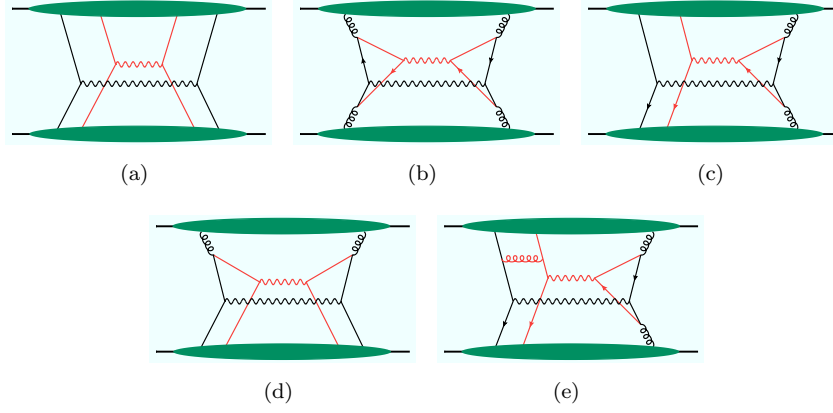
Fig. 2. Different contributions to the production of two electroweak gauge bosons: DPS (a), SPS (b) and their interference (c). Graphs (d) and (e) involve higher-twist distributions. Internal lines in the hard scattering are off shell by order Q . A vertical line for the final state cut is not shown for simplicity.
