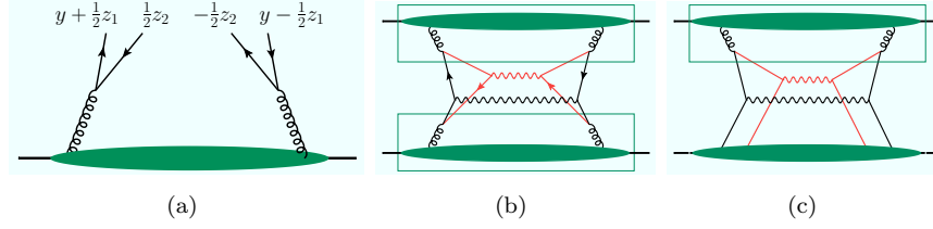
Fig. 4. Splitting provides a short-distance contribution to DPDs (a) and gives rise to 1v1 (b) and 2v1 (c) graphs for the DPS cross section. The boxes represent double parton distributions; partons emerging from them have virtualities much smaller than Q .
