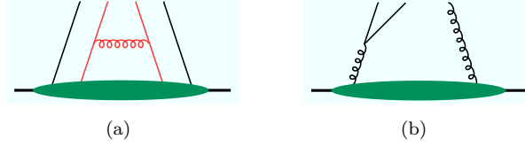
Fig. 7. (a) Ladder graph for a DPD. (b) Splitting contribution for a twist-three TMD.
