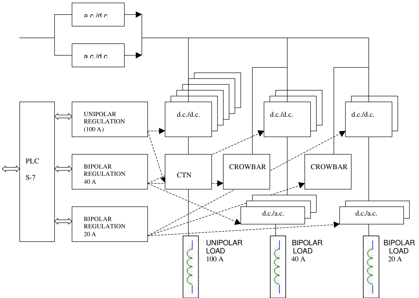
Fig. 2.: General schematic of the redundant power supplies for the Main Linac.
