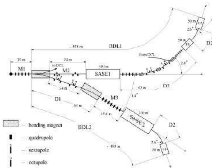
Fig. 8: Magnet lattice of the electron beam distribution system
