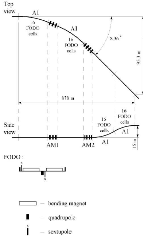
Fig. 7: Magnet lattice of the beam elevation system
