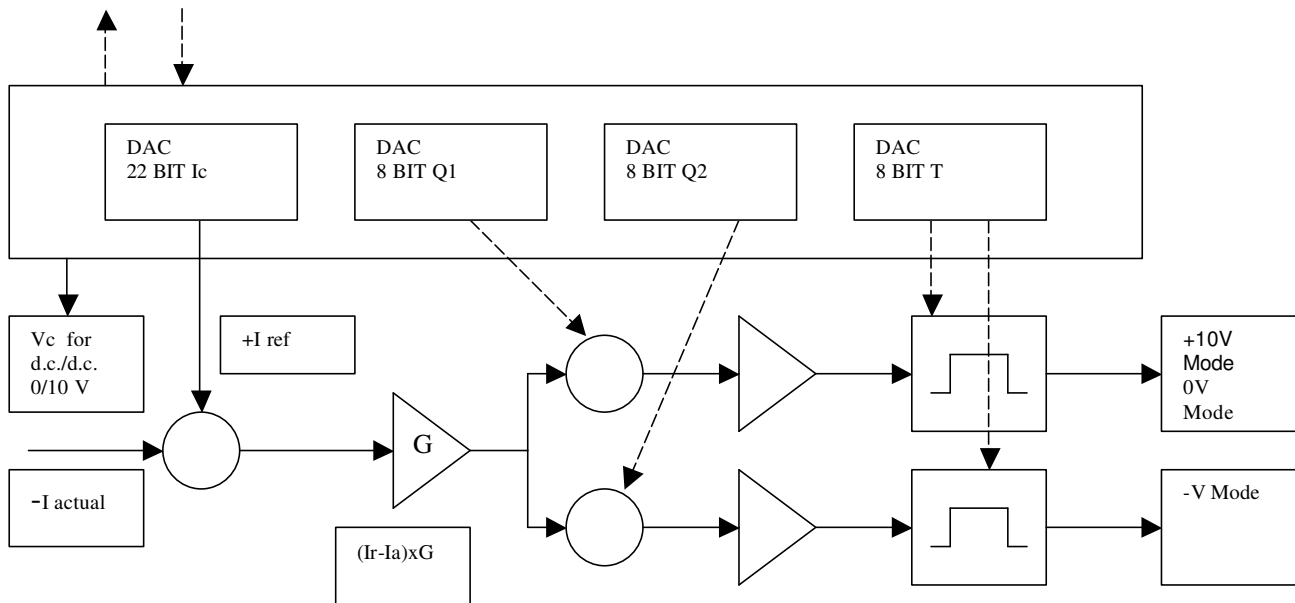
Figure 5.6.- Central Control System
