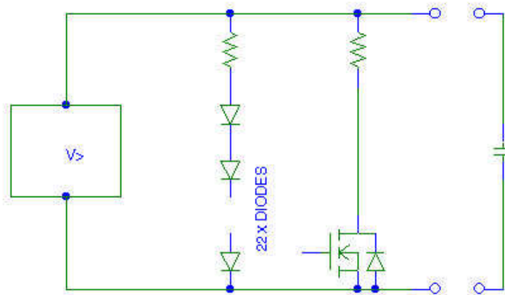
Figure 5.4.- Crowbar
