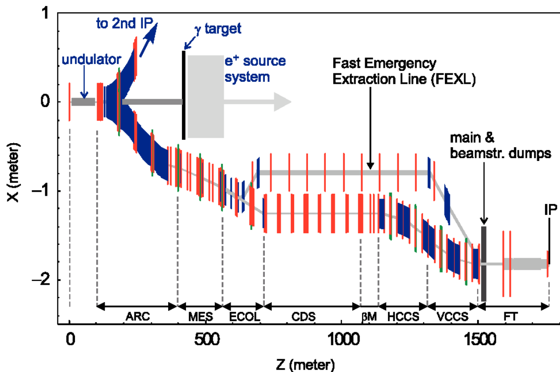
Fig. 10: Overview of the magnet lattice of the Beam delivery system
