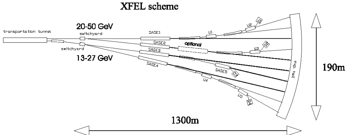
Fig. 5: General scheme of the XFEL
