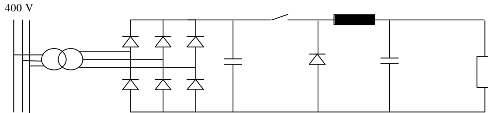
Fig.: 3 Schematic of the buck converter
