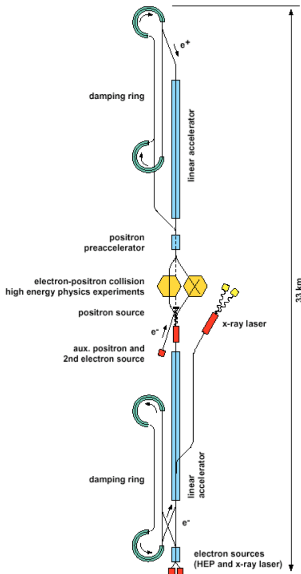
Fig.: 1 Principle overview of TESLA
