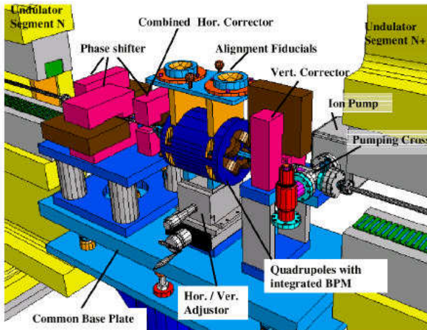
Fig. 6: View of undulator intersection
