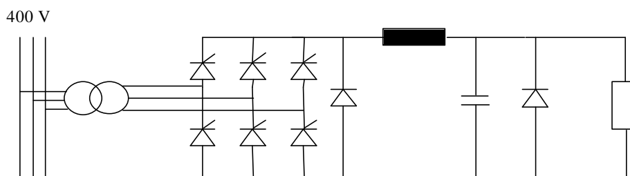
Fig. 4 Schematic of a 3 phase SRC bridge with passive filter
