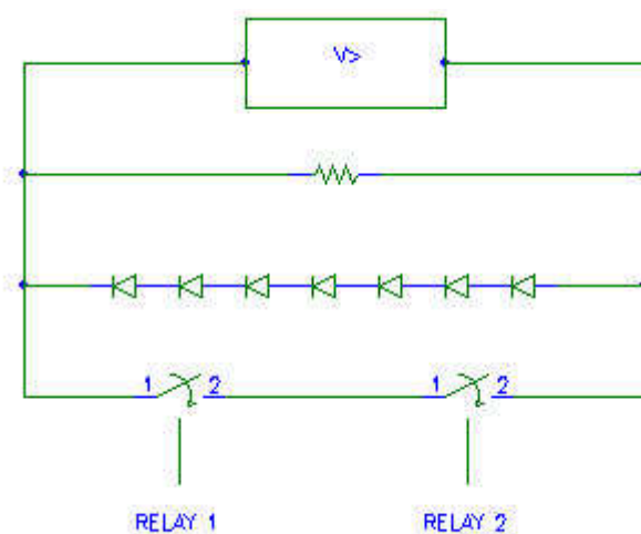
Figure 5.2 Negative Voltage Switch Module (NVS)
