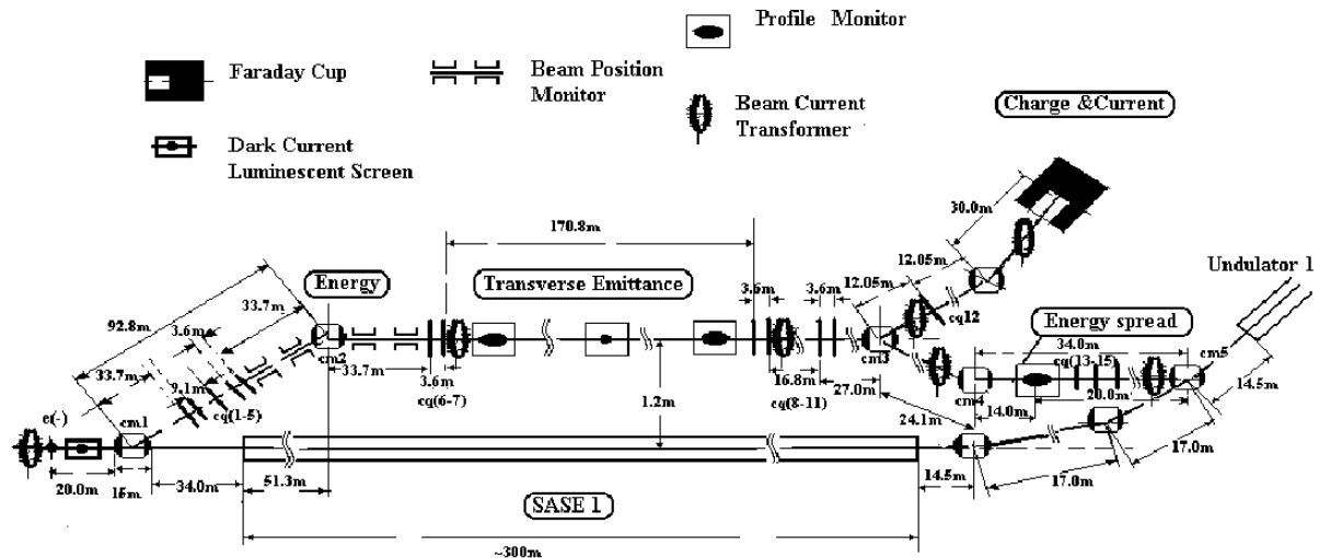
Fig. 9. Lattice of the diagnostic commissioning line
