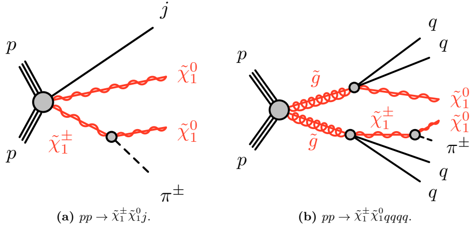
Figure 2. Example diagrams of the benchmark signal processes used in this analysis. In the case of direct chargino/neutralino production (a), the signal signature consists of a long-lived chargino, missing transverse momentum and initial-state radiation. In the case of the strong channel (b), each gluino decays into two quarks and a chargino or neutralino. A long-lived chargino, missing transverse momentum and multiple quarks, which are observed as jets, are the signatures of this signal.
