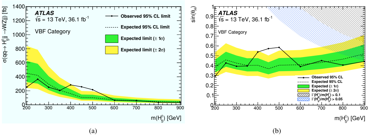
Figure 7: Observed and expected 95% CL upper limits on (a) \sigma \times \mathcal{B}(H_5^\pm \rightarrow W^\pm Z) and (b) the parameter \sin \theta_H of the GM Model as a function of m_{H_5^\pm} . The shaded region shows where the theoretical intrinsic width of the resonance would be larger than 5% or 10% of the mass.
