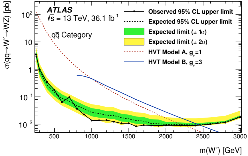
Figure 5: Observed and expected 95% CL upper limits on \sigma \times \mathcal{B}(W' \rightarrow W^\pm Z) for the q\bar{q} production of a W' boson in the HVT models as a function of its mass. The theoretical predictions for HVT Models A with g_V = 1 and B with g_V = 3 are also shown.
