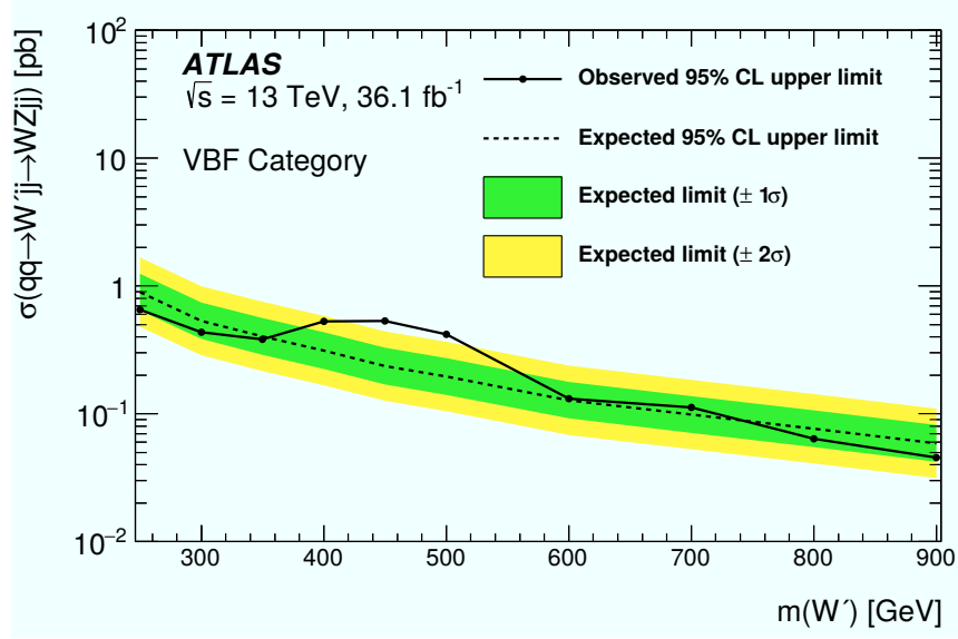
Figure 6: Observed and expected 95% CL upper limits on \sigma \times \mathcal{B}(W' \rightarrow W^\pm Z) for the VBF production of a W' boson in the HVT Model, with parameter c_F = 0 , as a function of its mass.
