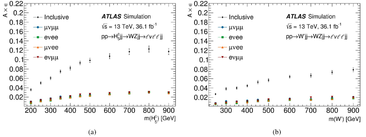
Figure 1: The signal selection acceptance times efficiency ( A \times \epsilon ), defined as the ratio of the number of MC signal events in the VBF category to the number of generated signal events, is presented as a function of the resonance mass. Figure 1(a) corresponds to the GM Model H_5^\pm while Figure 1(b) corresponds to the HVT models. The A \times \epsilon is shown for each decay channel and the sum of all lepton flavour combinations (inclusive). The error bars shown in each figure represent the total statistical and systematic uncertainties.
