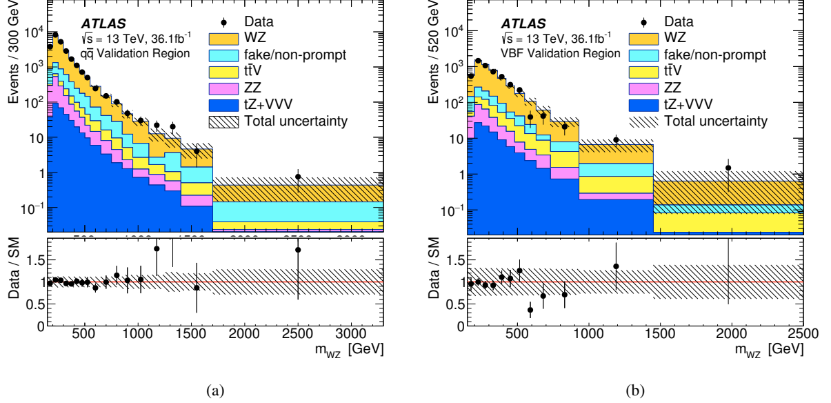
Figure 3: Observed and expected distributions of the WZ invariant mass in (a) the q\bar{q} validation region and (b) the VBF validation region. The points correspond to the data and the histograms to the expectations for the different SM processes. The uncertainty in the total background prediction, shown as bands, combines statistical, theory and systematic contributions. The bin sizes were chosen to reflect the resolution of a reconstructed signal, and the width of the previous to last bin is used to scale the bin contents. The last bin contains the overflow.
