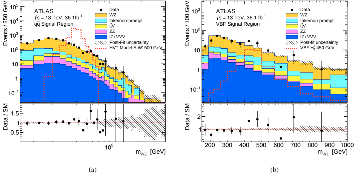
Figure 4: Observed and expected distributions of the WZ invariant mass (a) in the q\bar{q} and (b) in the VBF categories after applying all selection criteria. Signal predictions are overlaid, normalized to the predicted cross sections. The uncertainty in the total background prediction, shown as shaded bands, combines statistical, theory and systematic contributions. The lower panel show the ratios of the observed data to the background predictions.
