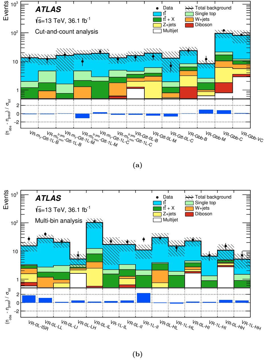
Figure 8. Results of the background-only fit extrapolated to the VRs of (a) the cut-and-count and (b) the multi-bin analyses. The t\bar{t} normalisation is obtained from the fit to the CRs shown in figure 7. The upper panel shows the observed number of events and the predicted background yield. All uncertainties defined in section 7 are included in the uncertainty band. The background category t\bar{t} + X includes t\bar{t}W/Z , t\bar{t}H and t\bar{t}t\bar{t} events. The lower panel shows the pulls in each VR.
