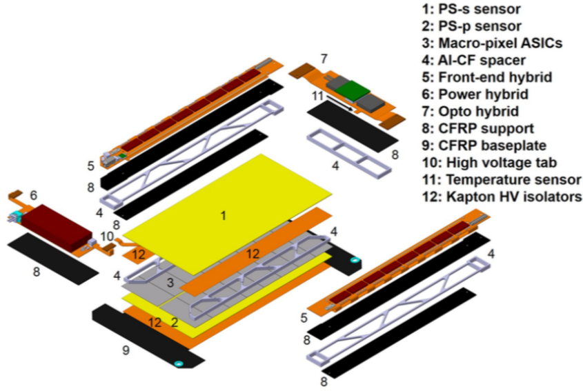
Figure 2: An exploded view of the PS module is shown with constituent parts indicated, taken from [1].
