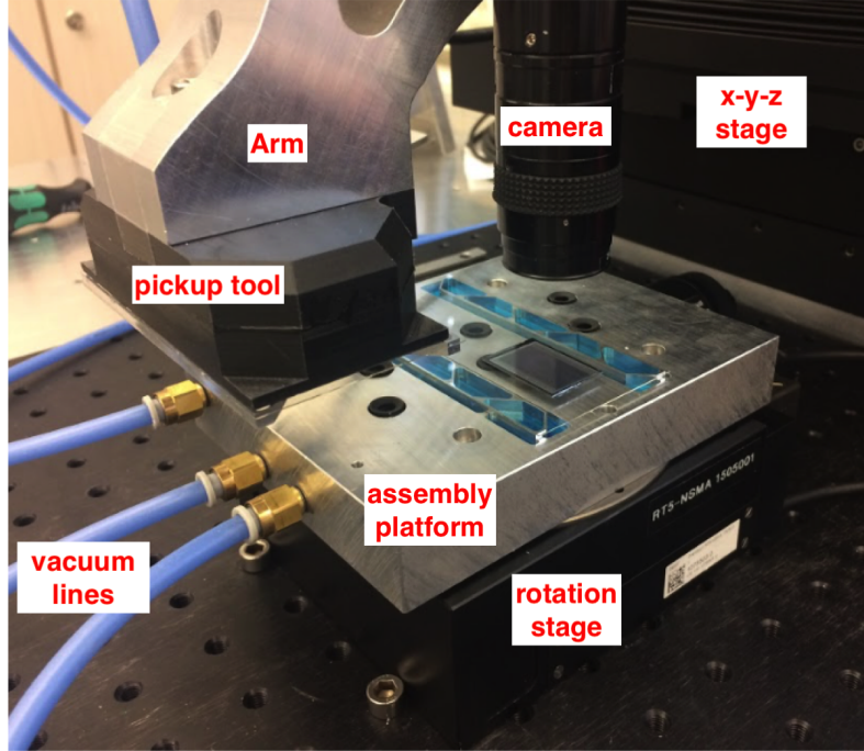
Figure 3: The hardware components of the assembly setup are shown.
