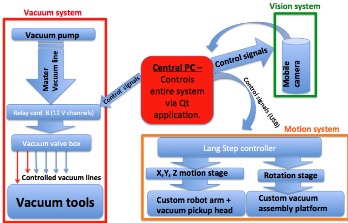
Figure 4: A schematic of the integration of the motion, vision and vacuum subsystems is shown.
