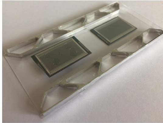
Figure 6: A prototype assembly is shown. The assembly consists of two dummy glass sensors with scrap silicon structures to provide fiducial markers and two dummy Al spacers.
