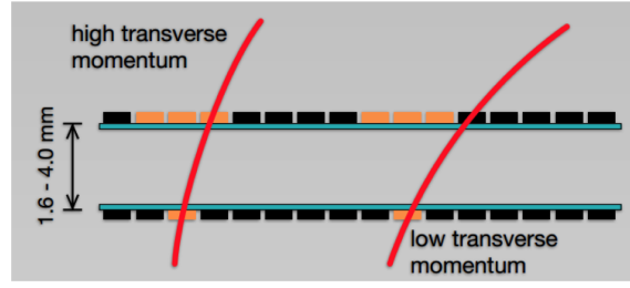
Figure 1: A schematic of the estimation of particle momentum in module volume is shown.
