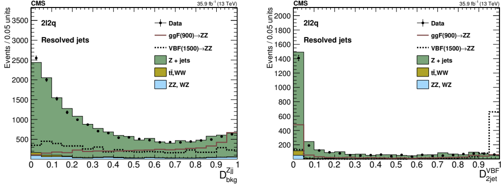
Figure 5. Distributions of the \mathcal{D}_{\text{bkg}}^{\text{Zij}} (left) and \mathcal{D}_{2\text{jet}}^{\text{VBF}} (right) discriminants in the signal region for the resolved selection. The points represent the data, the stacked histograms the expected background from simulation, and the open histograms the expected signal.
