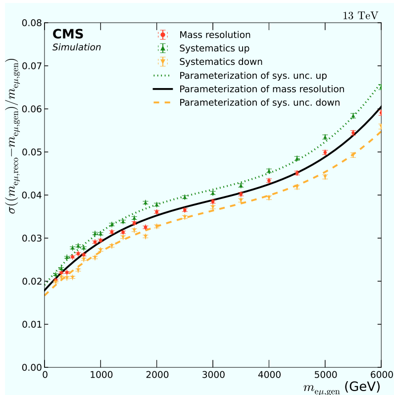
Figure 8. Relative mass resolution for all e\mu pairs, obtained through simulation of the RPV signal, from the reconstructed mass m_{e\mu, \text{reco}} and the generated mass m_{e\mu, \text{gen}} , as a function of the generated mass. The effect of the systematic uncertainties on the mass resolution is shown. The systematically shifted upper and lower mass resolutions are shown in the figure with the corresponding parameterization for the upward shifts in dotted green and the downward shifts in dashed orange.
