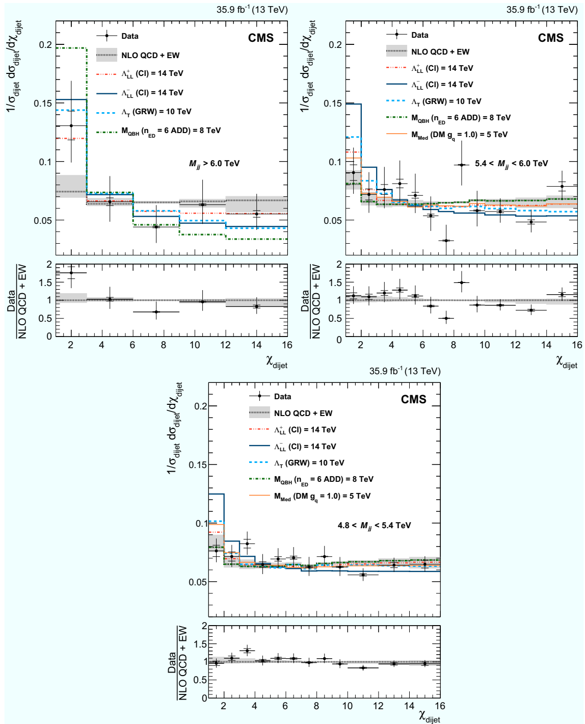
Fig. 1 Normalized \chi_{\text{dijet}} distributions in the three highest mass bins. Unfolded data are compared to NLO predictions (black dotted line). The error bars represent statistical and experimental systematic uncertainties combined in quadrature. The ticks on the error bars correspond
