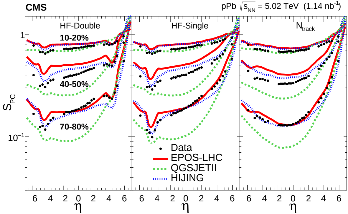
Figure 5: Ratio of peripheral to central E_T production, S_{PC} , as a function of \eta for three centrality ranges for HF-Double (left), HF-Single (middle), and N_{\text{track}} (right) for data, and for the EPOS-LHC, QGSJET II, and HIJING event generators. The systematic uncertainties are dominant and are of comparable size to the data points.
