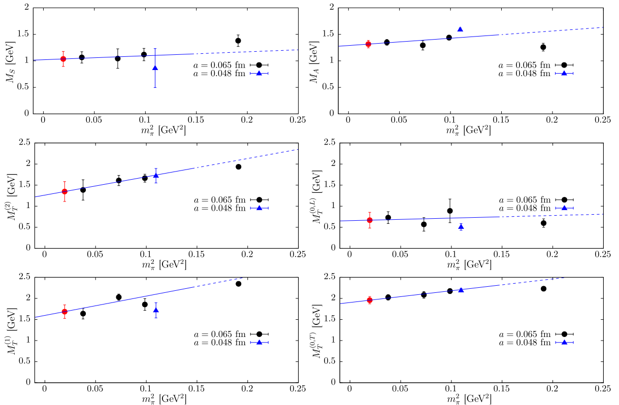
FIG. 9. Chiral extrapolations for each monopole and dipole mass, excluding the ensemble E5 with the largest pion mass. The blue point corresponds to the lattice ensemble N6 and gives an indication about discretization effects. Only the statistical error is displayed.
