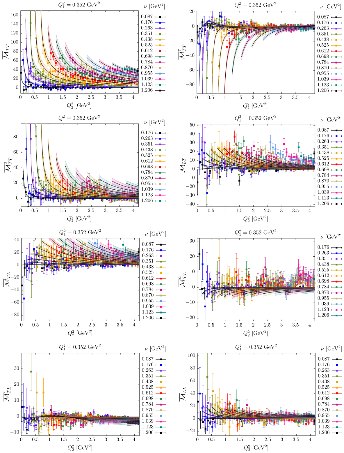
FIG. 10. The eight amplitudes ( \times 10^6 ) for the ensemble G8 and for Q_1^2 = 0.352 \text{ GeV}^2 . The curves with error bands represent the fit results discussed in Sec. VI.
