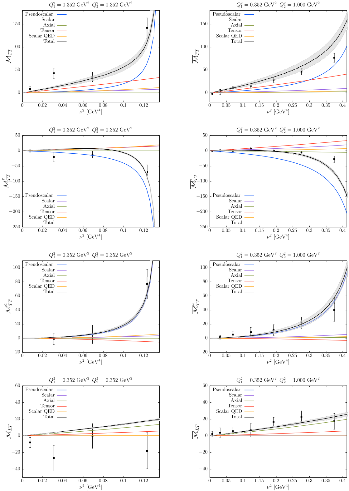
FIG. 6. The dependence of the amplitudes \overline{\mathcal{M}}_{TT} , \overline{\mathcal{M}}_{TT}^\tau , \overline{\mathcal{M}}_{TT}^a and \overline{\mathcal{M}}_{LT} ( \times 10^6 ) on \nu for two different values of Q_2^2 , the virtuality Q_1^2 = 0.352 \text{ GeV}^2 being fixed. The results correspond to the lattice ensemble G8. Note that at fixed photon virtualities, the form factors are completely determined. The black line corresponds to the total contribution and each colored line represents a single-meson contribution.
