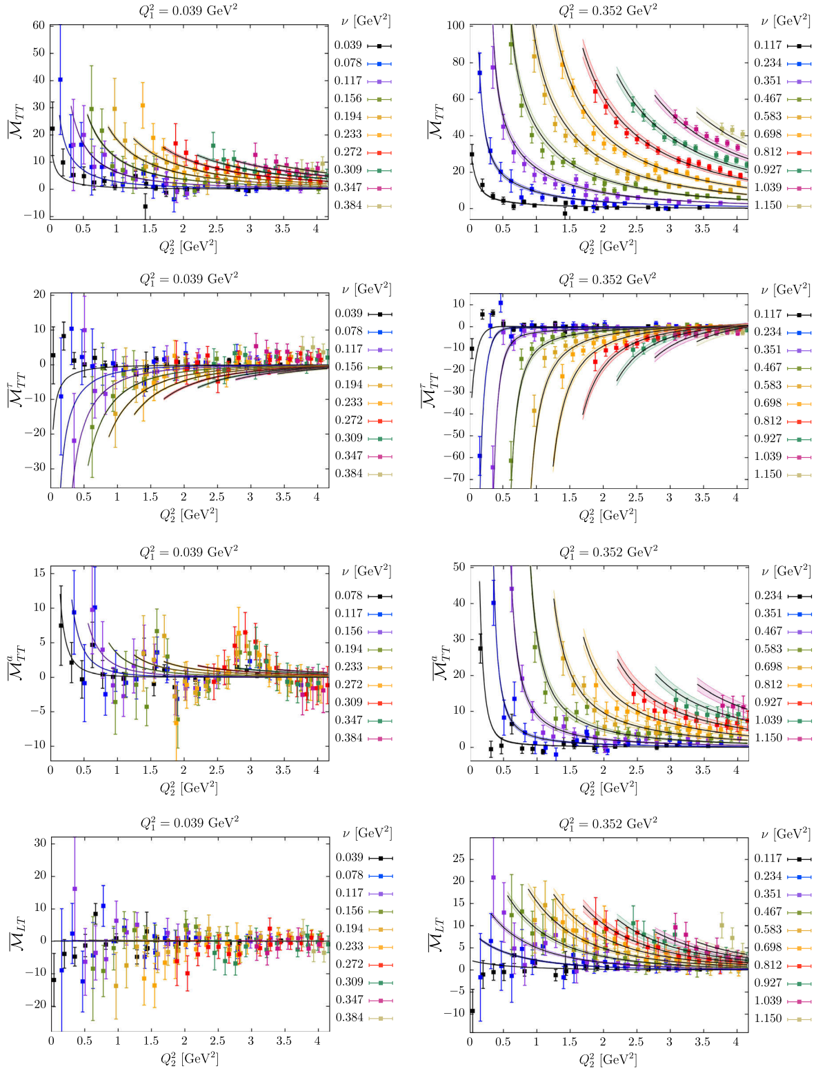
FIG. 3. Amplitudes \overline{\mathcal{M}}_{TT} , \overline{\mathcal{M}}_{TT}^\tau , \overline{\mathcal{M}}_{TT}^a and \overline{\mathcal{M}}_{LT} ( \times 10^6 ) for the ensemble F6 and for two different values of Q_1^2 (left: Q_1^2 = 0.039 \text{ GeV}^2 , right: Q_1^2 = 0.352 \text{ GeV}^2 ). The curves with error bands represent the fit results discussed in Sec. VI.
