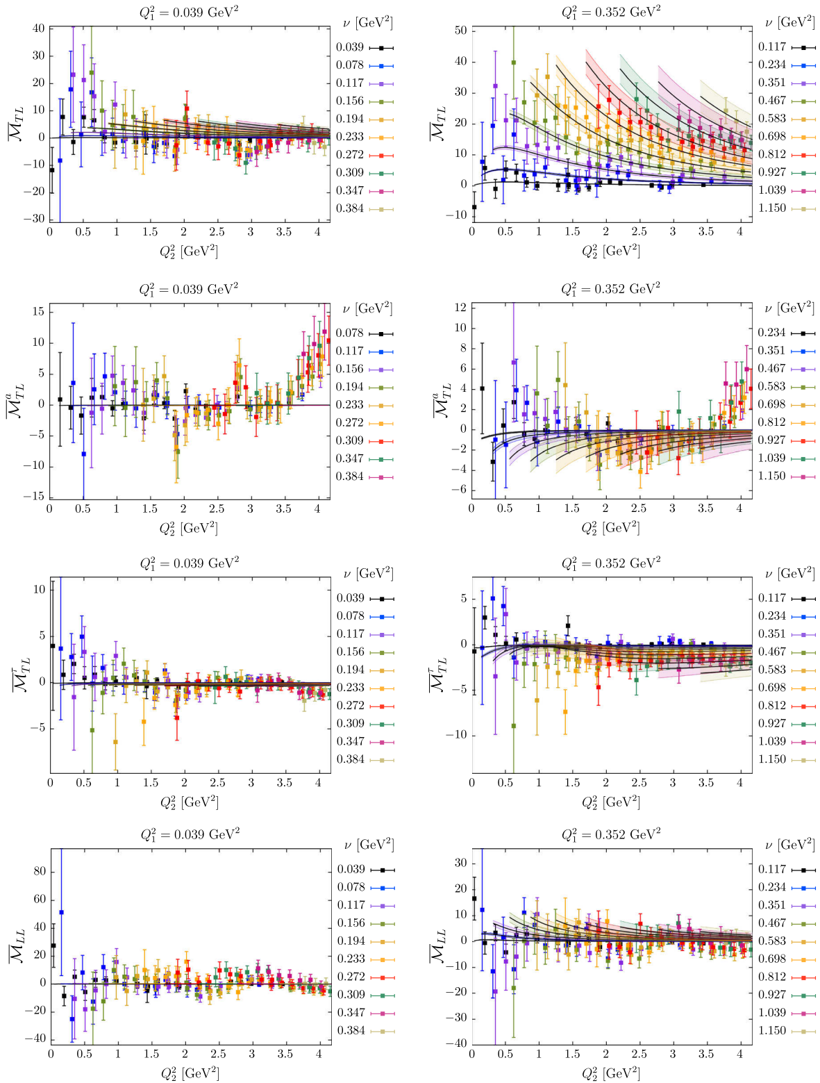
FIG. 4. Amplitudes \overline{\mathcal{M}}_{TL} , \overline{\mathcal{M}}_{TL}^a , \overline{\mathcal{M}}_{TL}^r and \overline{\mathcal{M}}_{LL} ( \times 10^6 ) for the ensemble F6 and for two different values of Q_1^2 (left: Q_1^2 = 0.039 \text{ GeV}^2 , right: Q_1^2 = 0.352 \text{ GeV}^2 ). The curves with error bands represent the fit results discussed in Sec. VI.
