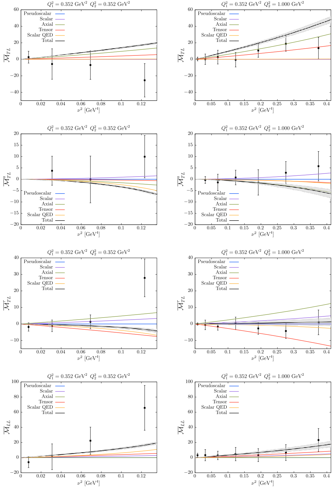
FIG. 7. The dependence of the amplitudes \overline{\mathcal{M}}_{TL} , \overline{\mathcal{M}}_{TL}^a , \overline{\mathcal{M}}_{TL}^r , \overline{\mathcal{M}}_{LL} ( \times 10^6 ) on \nu for two different values of Q_2^2 , the virtuality Q_1^2 = 0.352 \text{ GeV}^2 being fixed. The results correspond to the lattice ensemble G8. Note that at fixed photon virtualities, the form factors are completely determined. The black line corresponds to the total contribution and each colored line represents a single-meson contribution.
