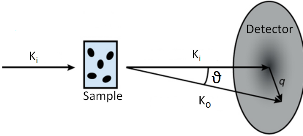
Figure 4.1: Representation of a scattering experiment. The incident X-ray beam with wave vector \mathbf{k}_i is scattered by the sample by the outgoing beam \mathbf{k}_o . The scattering angle between \mathbf{k}_i and \mathbf{k}_o is denoted as \vartheta .
