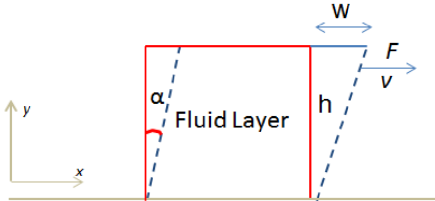
Figure 3.1: Illustration of a fluid deformation by a force F deforming the geometry by an angle \alpha and a length w . h is the height between the two adjacent layers of the fluid with a velocity v .
