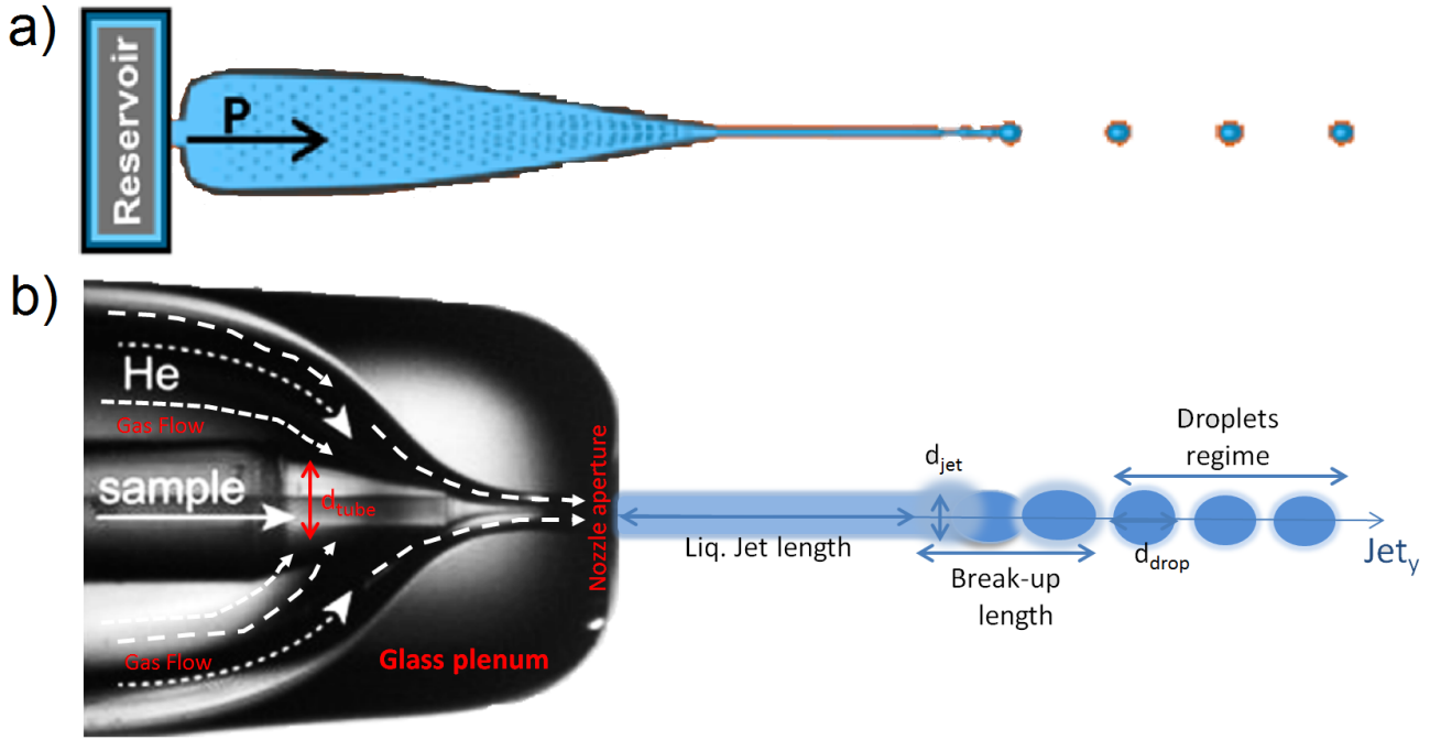
Figure 1.3: Scheme with two different kinds of liquid jets nozzles. a) Rayleigh nozzle, adapted from [2]. b) Glass GDVN Nozzle, d_{jet} and d_{drop} is the definition of jet and droplet diameter, respectively while d_{tube} is the inner tube diameter.
