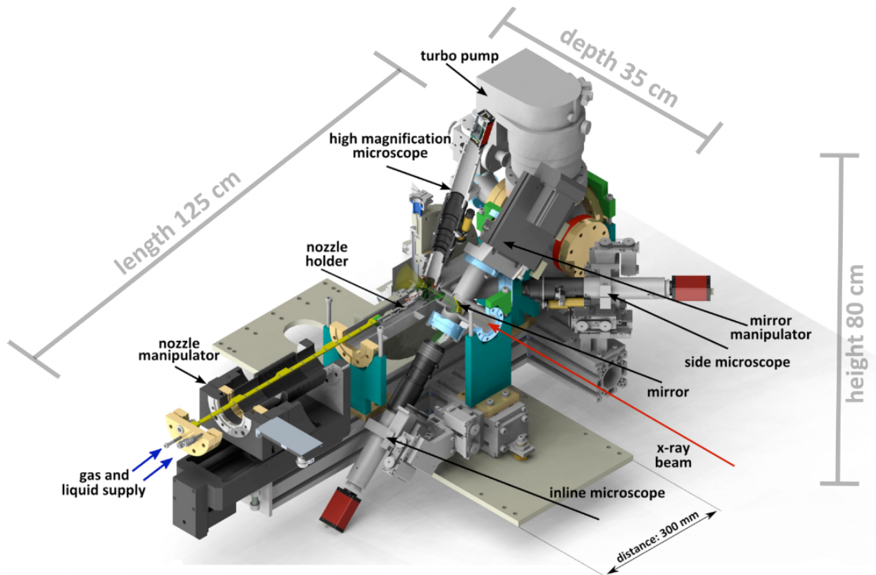
Figure 6.1: Liquid jet setup overview [14, 15]
