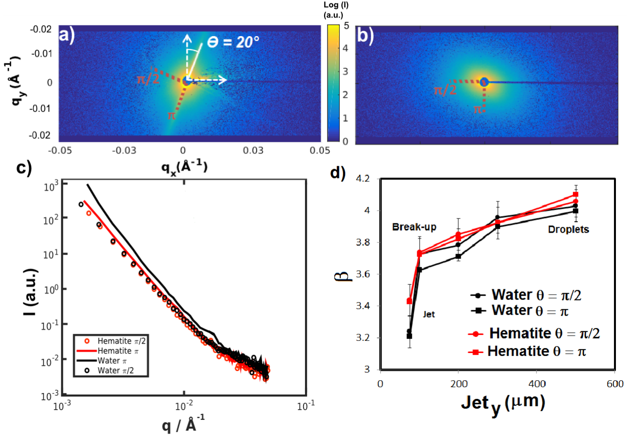
Figure 8.10: SAXS patterns from hematite dispersion acquired at the jet center and from different distance of nozzle tip: a) 75 \mu\text{m} and b) 500 \mu\text{m} , corresponding to jet and droplets regime respectively. The angle directions \theta = \pi and \theta = \pi/2 used for the data analysis are depicted in both patterns. c) A log-log plot of the integrated intensity I as a function of momentum transfer q taken at jet regime, 75 \mu\text{m} downstream the nozzle tip. The scattering curves of water and hematite dispersion presents the integration along the streak direction, \theta = \pi , and perpendicular to it ( \theta = \pi/2 ). d) Comparison of q -dependencies measured at different distances along the jet for water and hematite dispersion along the different depicted angles.
