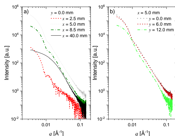
Figure 1 Examples of X-ray scattering curves with subtracted background: a) at different axial distances x from the magnetron target and at the radial distance of y = 0.0 \text{ mm} (on the GAS axis); b) at different radial distances and at the axial distance of x = 5.0 \text{ mm} .
