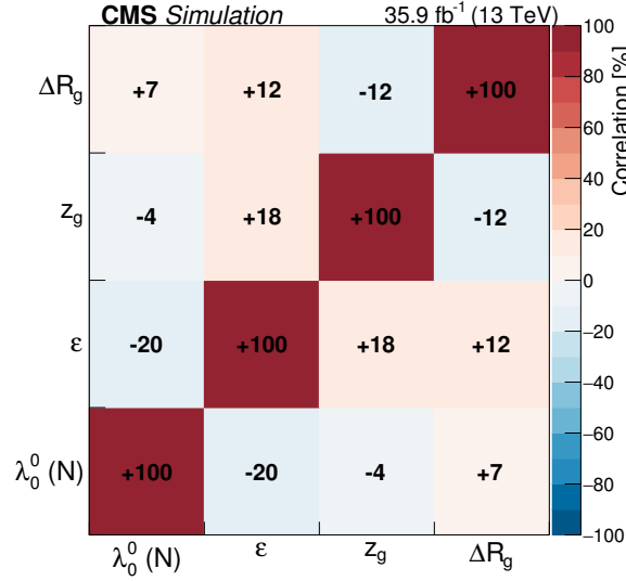
Figure 21: Correlations of the jet-substructure observables used in this analysis obtained at the particle level for the set of four minimally correlated observables.
