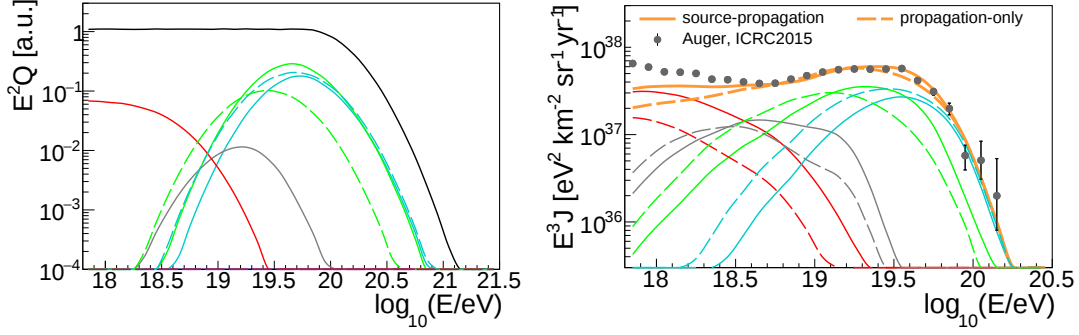
Figure 1. Comparison between propagation-only model (dashed curves), corresponding to Zhang et al. (2018), and source-propagation model (solid curves), including the nuclear disintegration in the source corresponding to Biehl et al. (2018a), for the same injection composition and parameters. Left: Cosmic-ray fluxes escaping from the source (multiplied by E^2 ). Dashed curves refer to the spectra coming out of the source given by Eq. (7) in Zhang et al. (2018) (green A = 16 and cyan A = 28 ). Solid curves refer to a power law acceleration spectrum \propto E^{-2} \exp(-E/E_{\max}) (black curve, sum of 60% A = 16 and 40% A = 28 ) injected within the source and to the groups of isotopes generated by the interactions in the source (red A = 1 , grey 2 \leq A \leq 4 , green 5 \leq A \leq 24 , cyan 25 \leq A \leq 28 ). Right: Cosmic-ray fluxes at detection (multiplied by E^3 ). The isotope groups are defined as reported above. The plots are obtained using the parameters corresponding to the best-fit as reported in Fig. 3, and are independently normalized to the UHECR flux.
