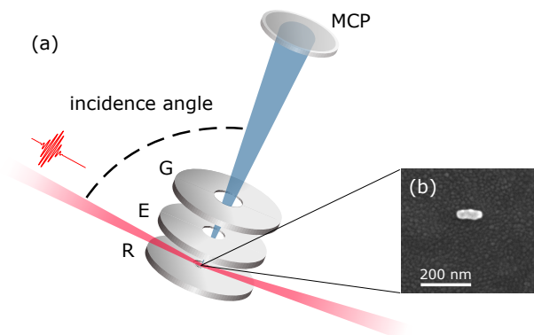
Figure 1: (a) VMI spectrometer consisting of three electrodes: repeller (R), extractor (E) and ground (G); (b) SEM image of the 75-μm pitch field-emitter array of Au nanorods.
