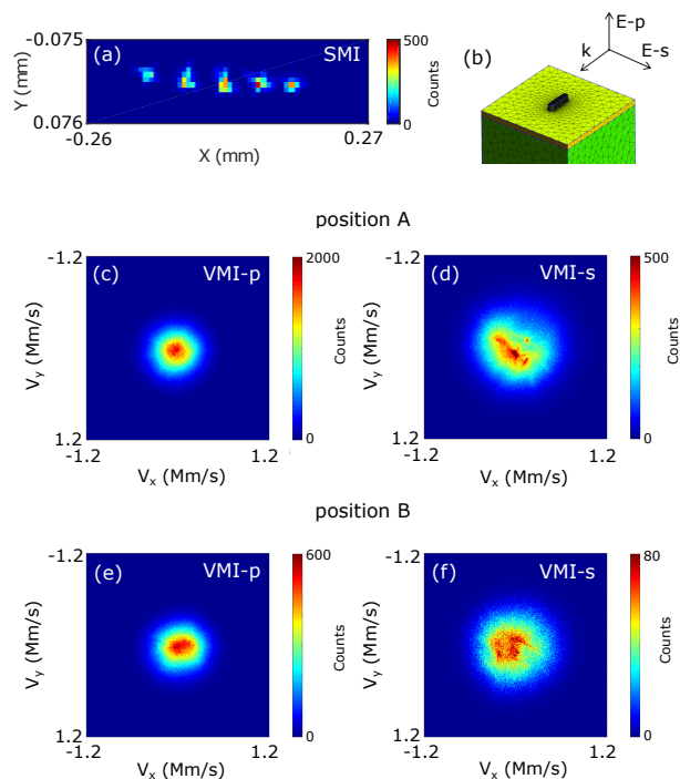
Figure 2: (a) SMI image of a 75-μm pitch field-emitter array of Au nanorods; (b) sketch of laser polarization with respect to the experiment, where E-p and E-s denote the electric field directions under p- and s-polarization, respectively; VMI images of position A under (c) p-polarization and (d) s-polarization; VMI images of position B under (e) p-polarization and (f) s-polarization.
