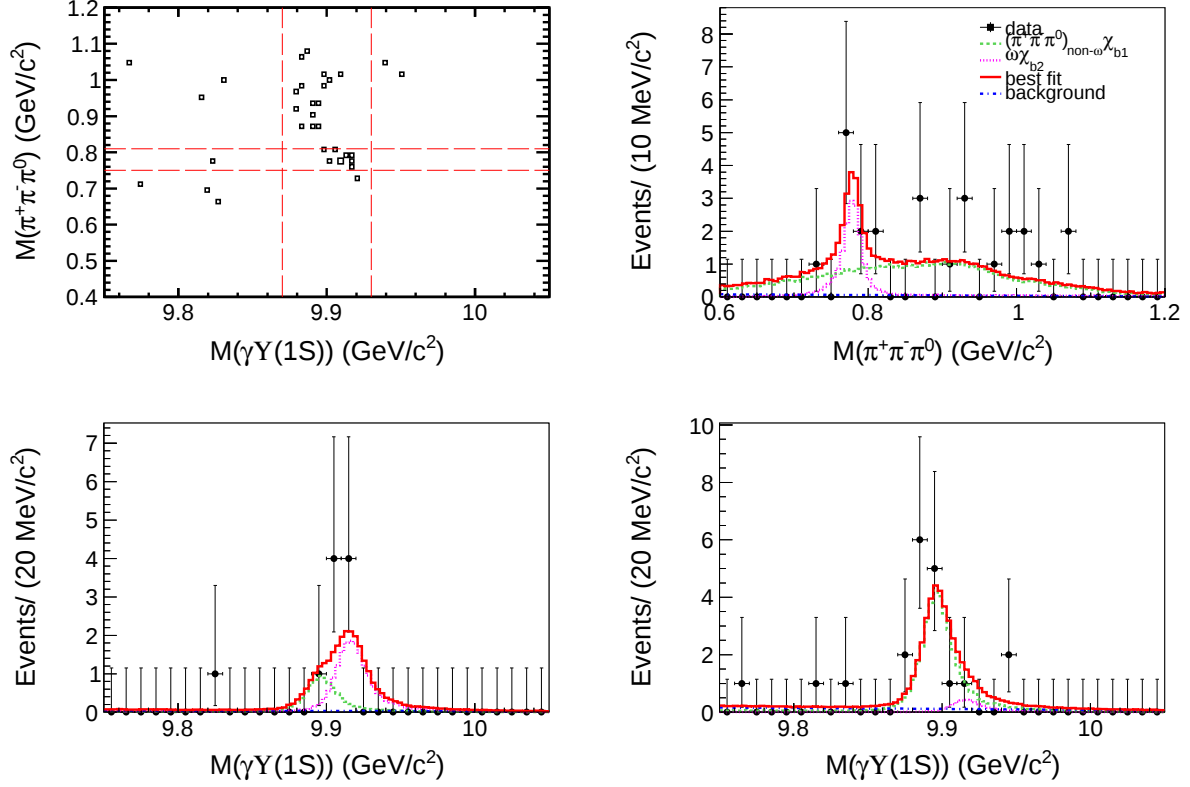
FIG. 1. A scatter plot of M(\pi^+\pi^-\pi^0) versus M(\gamma\Upsilon(1S)) from data (top left), and the projections of the 2D fit for events in \chi_{bJ} signal region (top right), in \omega signal region (bottom left), and out of \omega signal region (bottom right). Points with error bars are data, solid lines are the best fit, dashed lines are the \chi_{b1} signals, dotted lines are \chi_{b2} signals, and the dash-dotted lines are the fitted background.
