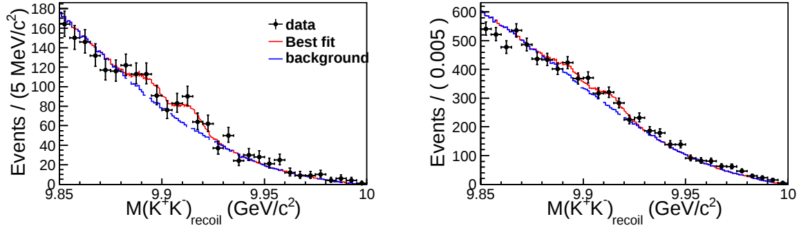
FIG. 3. The simultaneous fit results for data having M(\gamma K^+ K^-) in the \Upsilon(1S) mass window (left) and out (right). Dots with error bars are data, the red solid lines are the best fit, and blue dashed lines are backgrounds.
