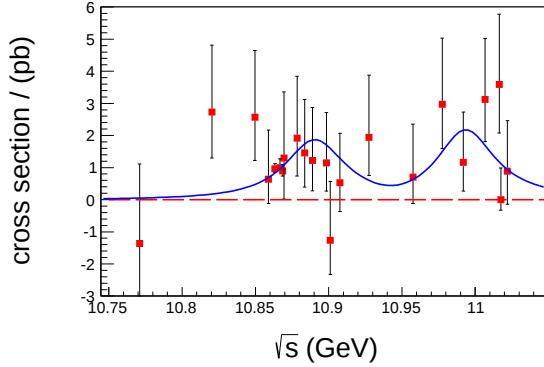
FIG. 2. Fitting to the cross sections of e^+e^- \rightarrow \pi^+\pi^-\pi^0\chi_{bJ} . Red boxes with error bars are the cross sections of e^+e^- \rightarrow \pi^+\pi^-\pi^0\chi_{bJ} and solid blue curve is fitting curve.
