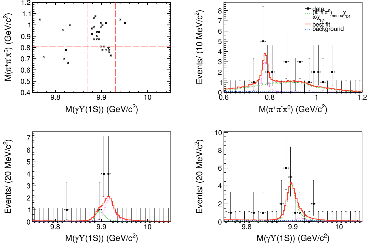
FIG. 1. A scatter plot of M(\pi^+\pi^-\pi^0) versus M(\gamma Y(1S)) from data (top left), and the projections of the 2D fit for events in \chi_{bJ} signal region (top right), in \omega signal region (bottom left), and out of \omega signal region (bottom right). Points with error bars are data, solid lines are the best fit, dashed lines are the \chi_{b1} signals, dotted lines are \chi_{b2} signals, and the dash-dotted lines are the fitted background.
