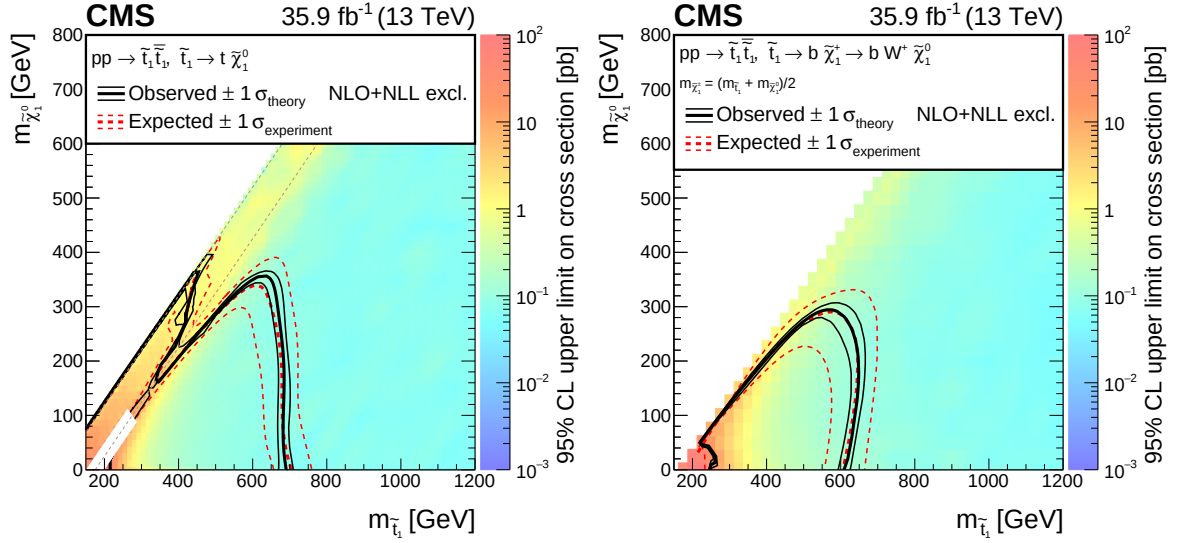
Figure 9: Upper limits at 95% CL on the top squark production cross section as a function of the top squark and neutralino masses. The plot on the left shows the results when top squark decays into a top quark and a neutralino are assumed. The two diagonal gray dashed lines enclose the compressed region where m_W < m_{\tilde{t}_1} - m_{\tilde{\chi}_1^0} \lesssim m_t . The plot on the right gives the limits for top squarks decaying into a bottom quark and a chargino, with the latter successively decaying into a W boson and a neutralino. The mass of the chargino is assumed to be equal to the average of the top squark and neutralino masses. Exclusion regions in the plane (m_{\tilde{t}_1}, m_{\tilde{\chi}_1^0}) are determined by comparing the upper limits with the NLO+NLL production cross sections. The thick dashed red line shows the expected exclusion region. The thin dashed red lines show the variation of the exclusion regions due to the experimental uncertainties. The thick black line shows the observed exclusion region, while the thin black lines show the variation of the exclusion regions due to the theoretical uncertainties in the production cross section.
